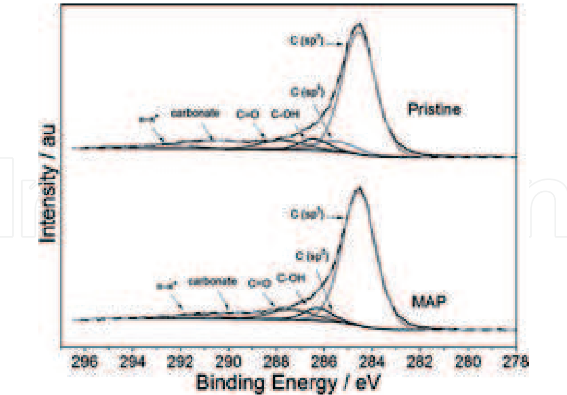
Figure 8. XPS of C1s spectrum of pristine CNTs (top spectrum) and oxidized/purified CNTs (bottom spectrum). Reproduced with a permission from Ref. [15].
