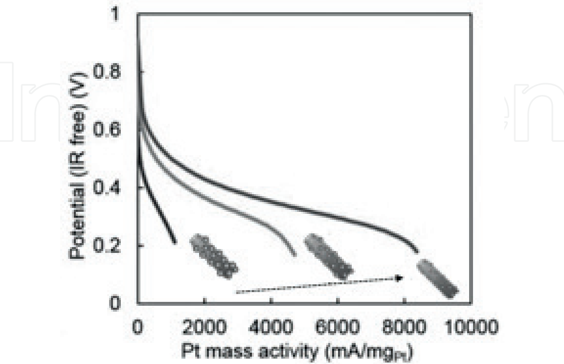
Figure 17. Potential curves as a function of platinum (Pt) mass activity. Reprinted with a permission from Ref. [31].
