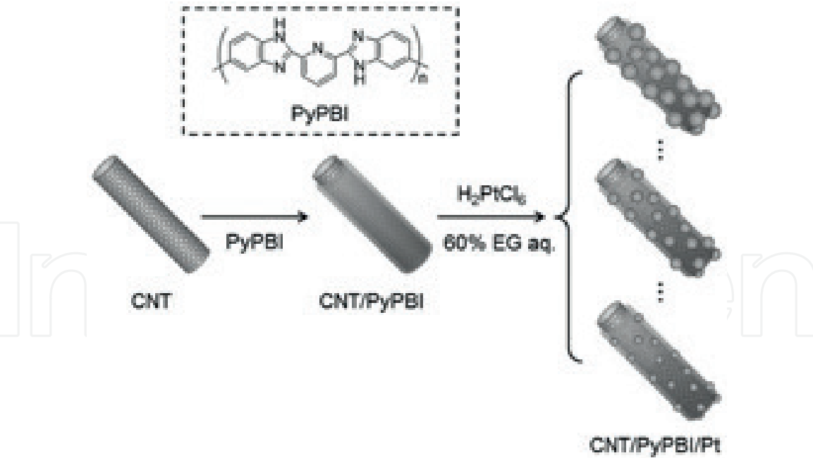
Figure 16. Schematic illustration of polymer wrapping and platinum deposition on CNTs. The figure shows how the authors have controlled the deposition of the platinum nanoparticles. Reprinted with a permission from Ref. [31].
