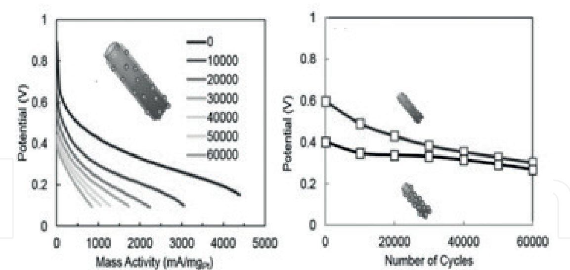
Figure 18. Durability potential curve test using MEA10 (small platinum nanosize). The polarization curves were measured after every 1000 cycles. For convenience, the data were plotted every 10,000 cycles (c). Plots of the cell voltage at 200 mA mgPt-1 for the MEA50 and MEA10.
