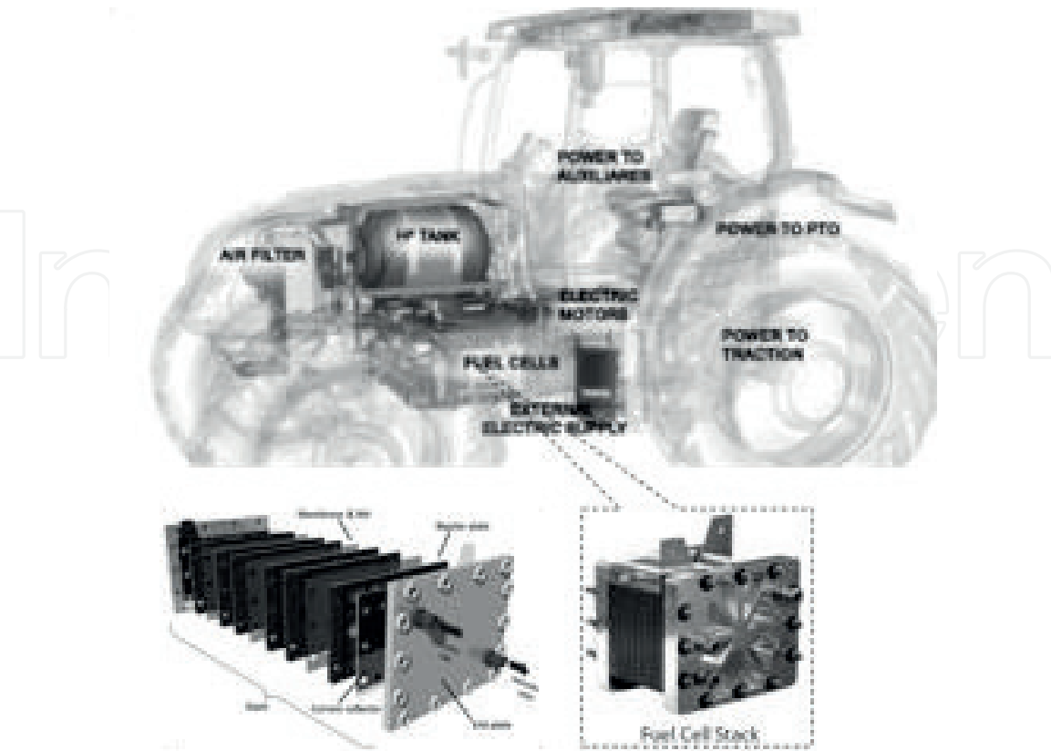
Figure 19. Schematic illustration of fuel cell tractor built by New Holland (photo courtesy of New Holland). The fuel cell stack depends on the required power.
