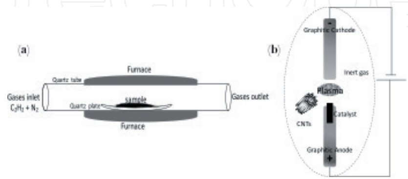
Figure 2. Schematic illustration of (a) CVD method for preparation of CNTs and (b) arc-discharge method for preparation of CNTs.
