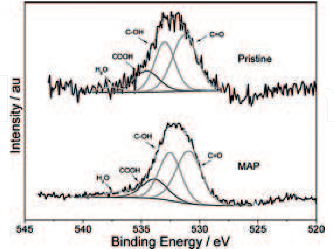
Figure 9. XPS of O1s spectrum of pristine CNTs (top spectrum) and oxidized/purified CNTs (bottom spectrum). Reproduced with a permission from Reference.
