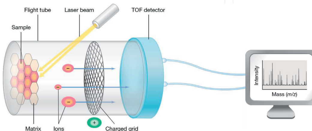
Figure 11. MALDI-TOF mass spectrometry device [11].
