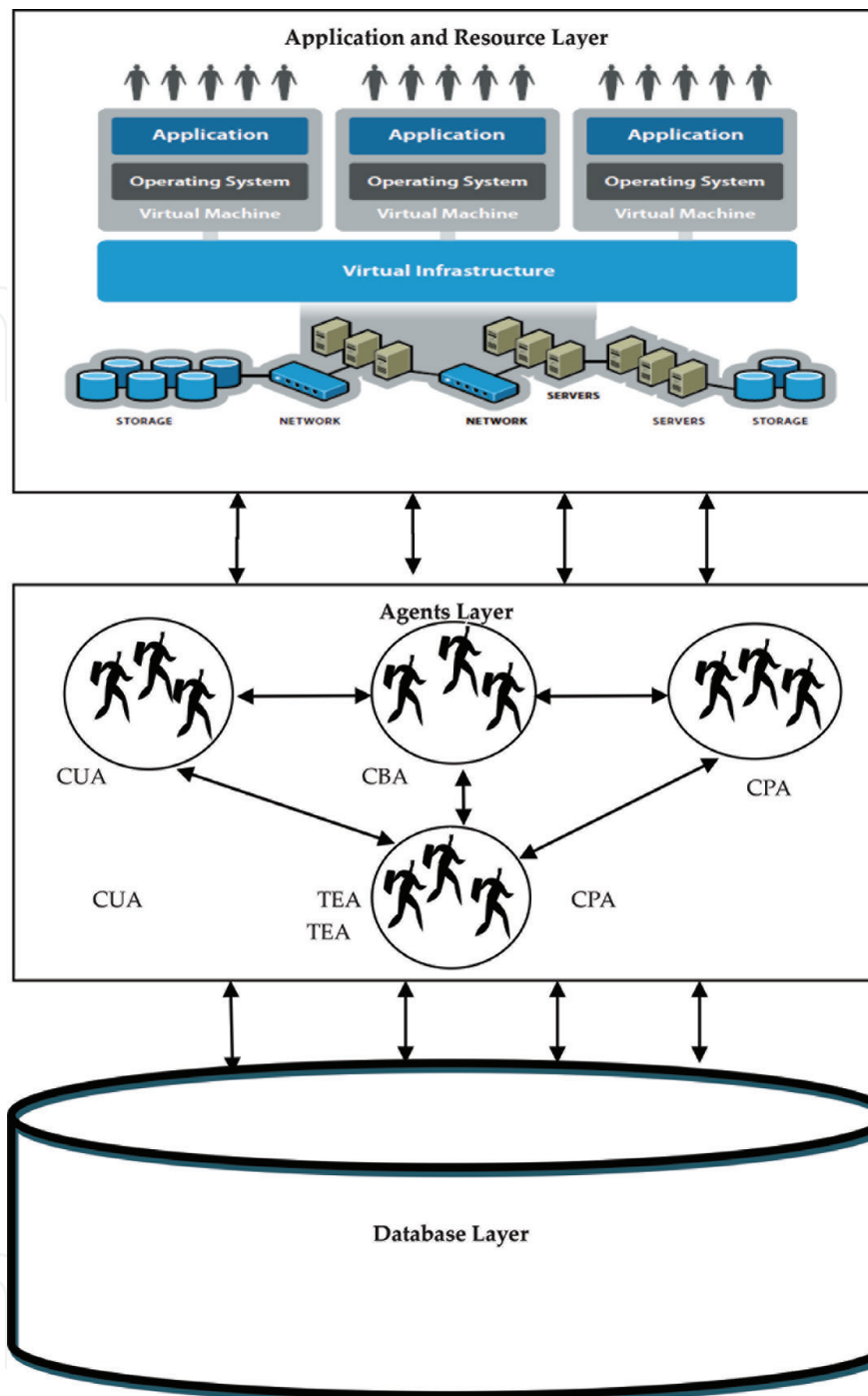
Figure 3. System architecture [32].
