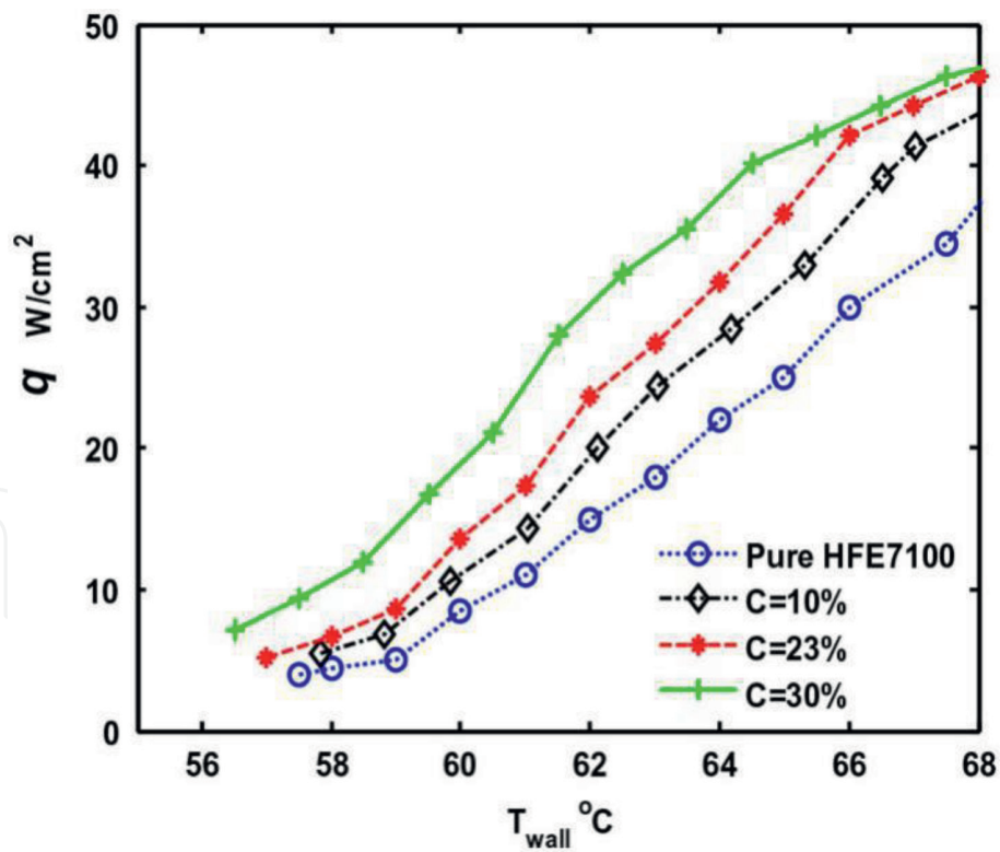
Figure 10. HFE7100 jet impingement (56–68°C) heat flux at the flow rate of 7.15 cc/s; (note: the inlet T_{\text{in}} was controlled at 56°C, nozzle: TGo.76, H = 20 \text{ mm} ). Slurry with 30% particle mass fraction improved average heat transfer coefficient by 70% when compared to pure HFE7100 for jet impingement at the temperature range from 62 to 66°C.
