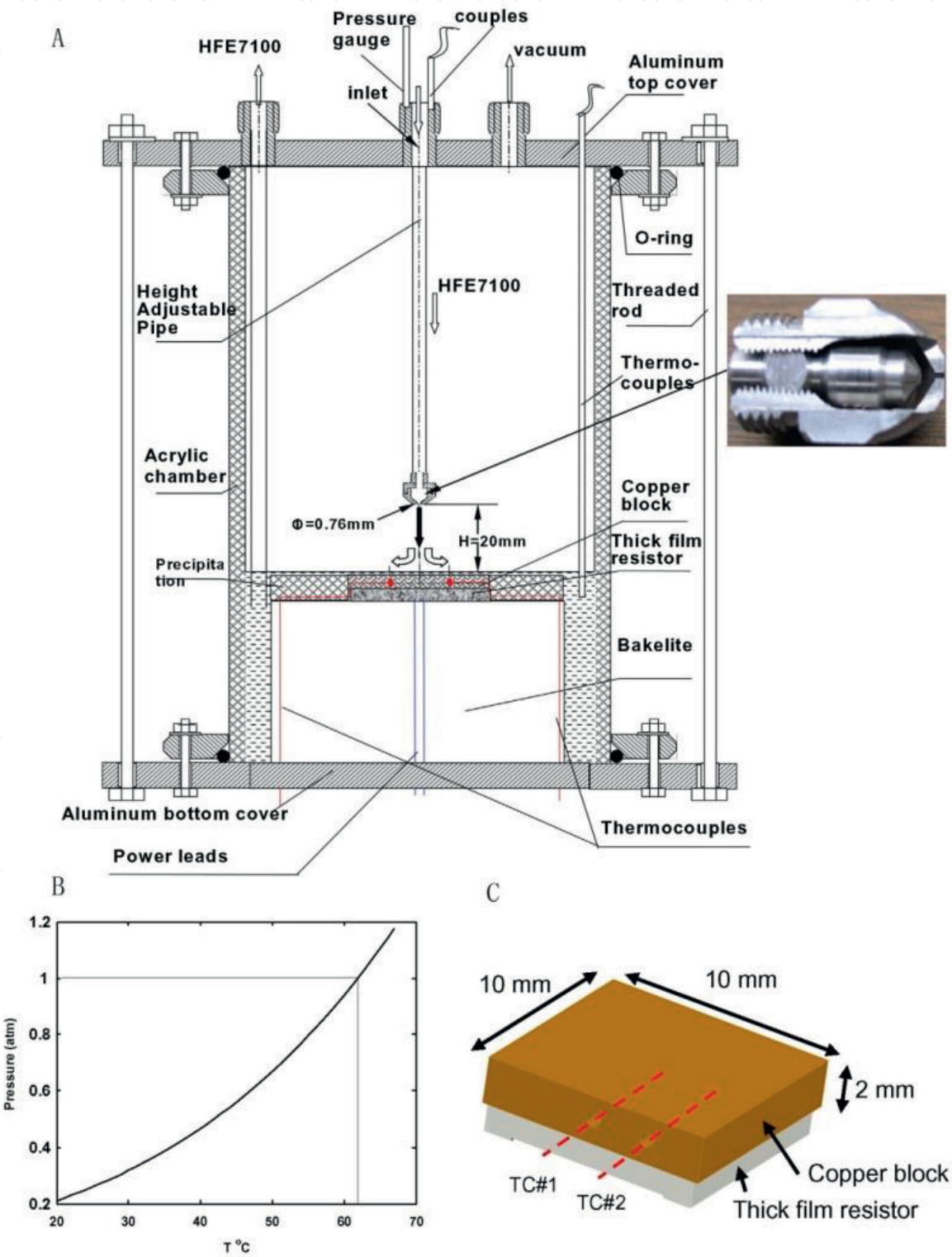
Figure 6. Illustrated scheme of test chamber (A) temperature vs. pressure of HFE7100 (B) and heater (C).
