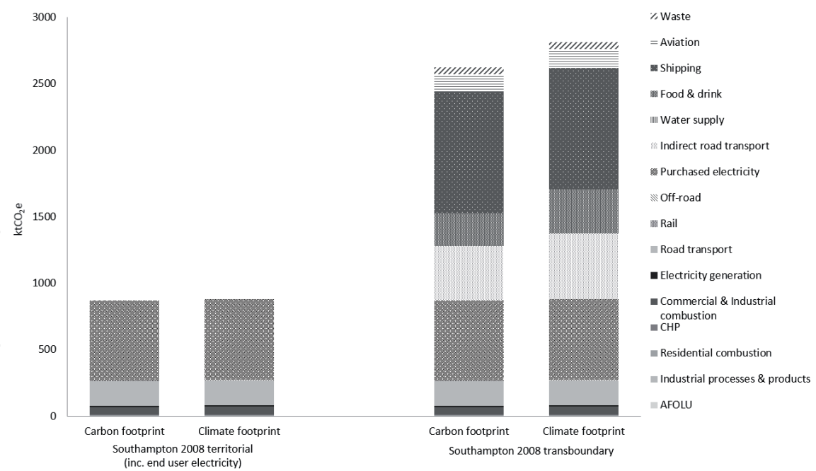
Figure 1. Comparison of case study territorial and transboundary carbon ( \text{CO}_2 , \text{CH}_4 ) and climate (Kyoto Basket) footprints.
