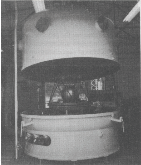
Figure 7. Entire system EM testing vacuum chamber [1].
