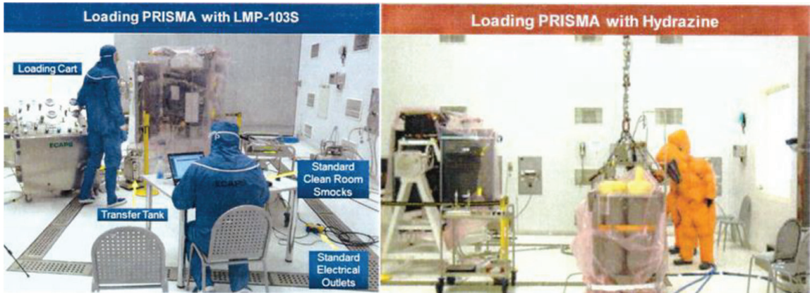
Figure 8. Propellant loading of satellite Prisma [20].
