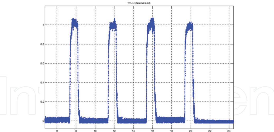
Figure 11. NewRocket engine operation in pulses.
