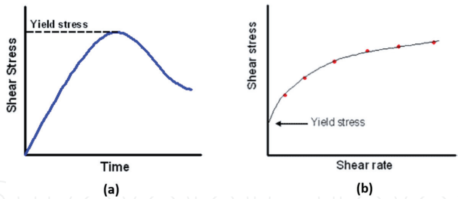
Figure 15. Common methods for measuring yield stress [56]. (a) Shearing a fluid at a low and constant shear rate and measuring the shear stress as a function of time and (b) extending the shear stress vs. shear rate curve at low shear rates.
