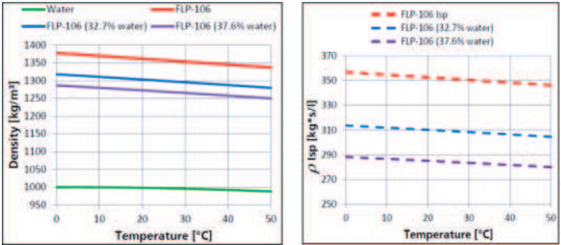
Figure 5. Density and \rho Isp as a function of temperature for water and FLP-106 with various values of water content [45].
