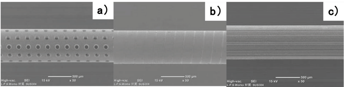
Figure 34. Microtexturing into the metallic tube. (a) Microdrilling of holes with the diameter of 100 \mu\text{m} into a AISI304 stainless steel pipe with D_{out} = 0.7 \text{ mm} and D_{in} = 0.58 \text{ mm} , (b) microgrooving of shallow grooves with the width of 25 \mu\text{m} and the depth of 3 \mu\text{m} into the same pipe as (a), and (c) microgrooving of lateral grooves with the depth of 30 \mu\text{m} into the same pipe as (a).
