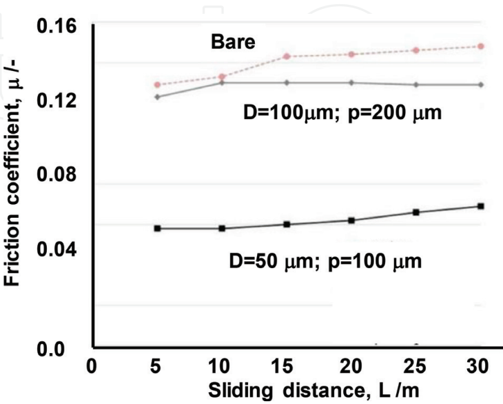
Figure 30. Variation of the friction coefficient with increasing the sliding distance for three cases; the bare die without microdimples, and the microdimpled dies with D = 100\text{ }\mu\text{m} and p = 200\text{ }\mu\text{m} and D = 50\text{ }\mu\text{m} and p = 100\text{ }\mu\text{m} , respectively.
