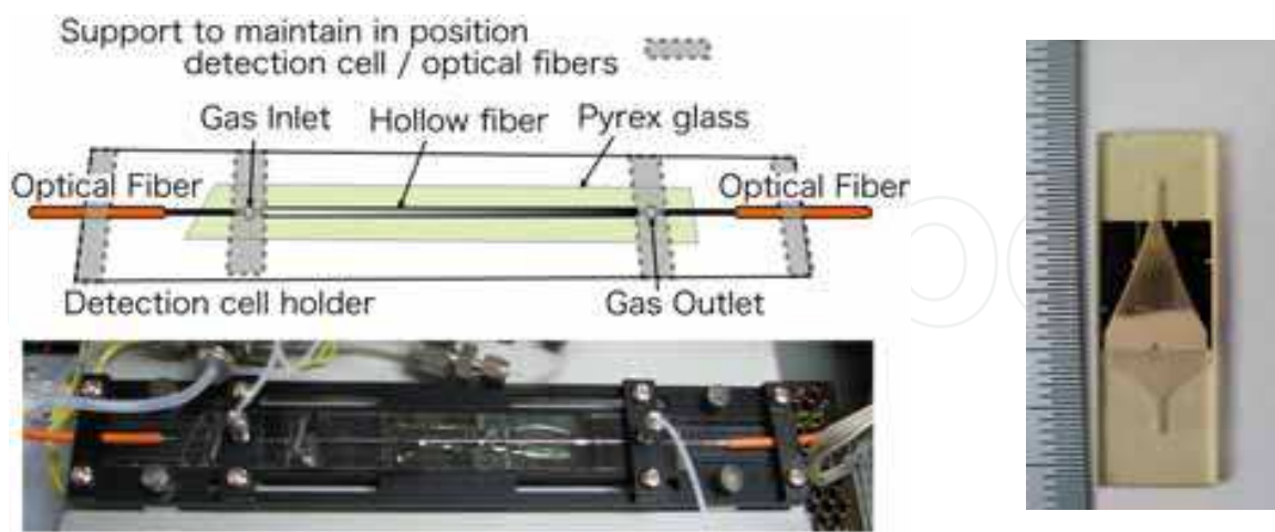
Fig. 2. Pictures of (left) the detection cell (10-cm-long light path) on its holder and (right) a micro-fabricated concentration cell half-filled with adsorbent (platinum heater electrodes on the rear side).
