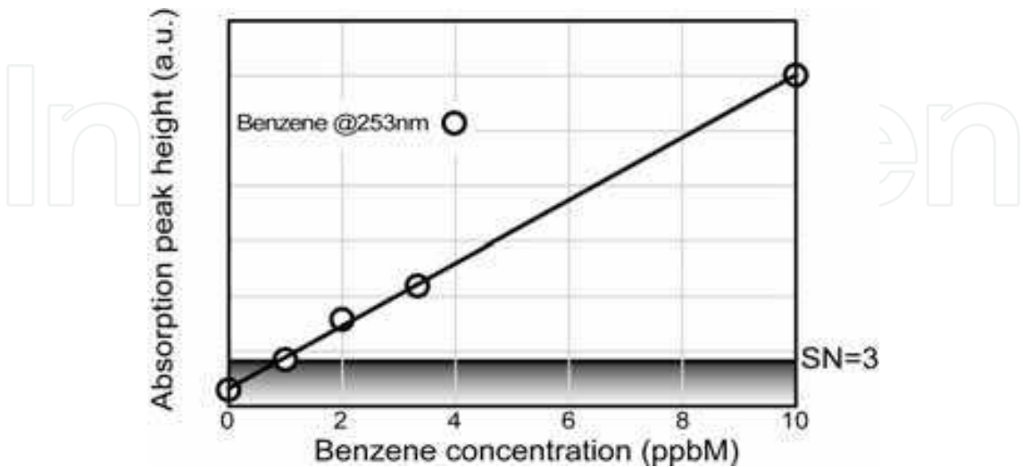
Fig. 3. Sensor response versus benzene concentration of calibrated gas mixture in dried nitrogen.
