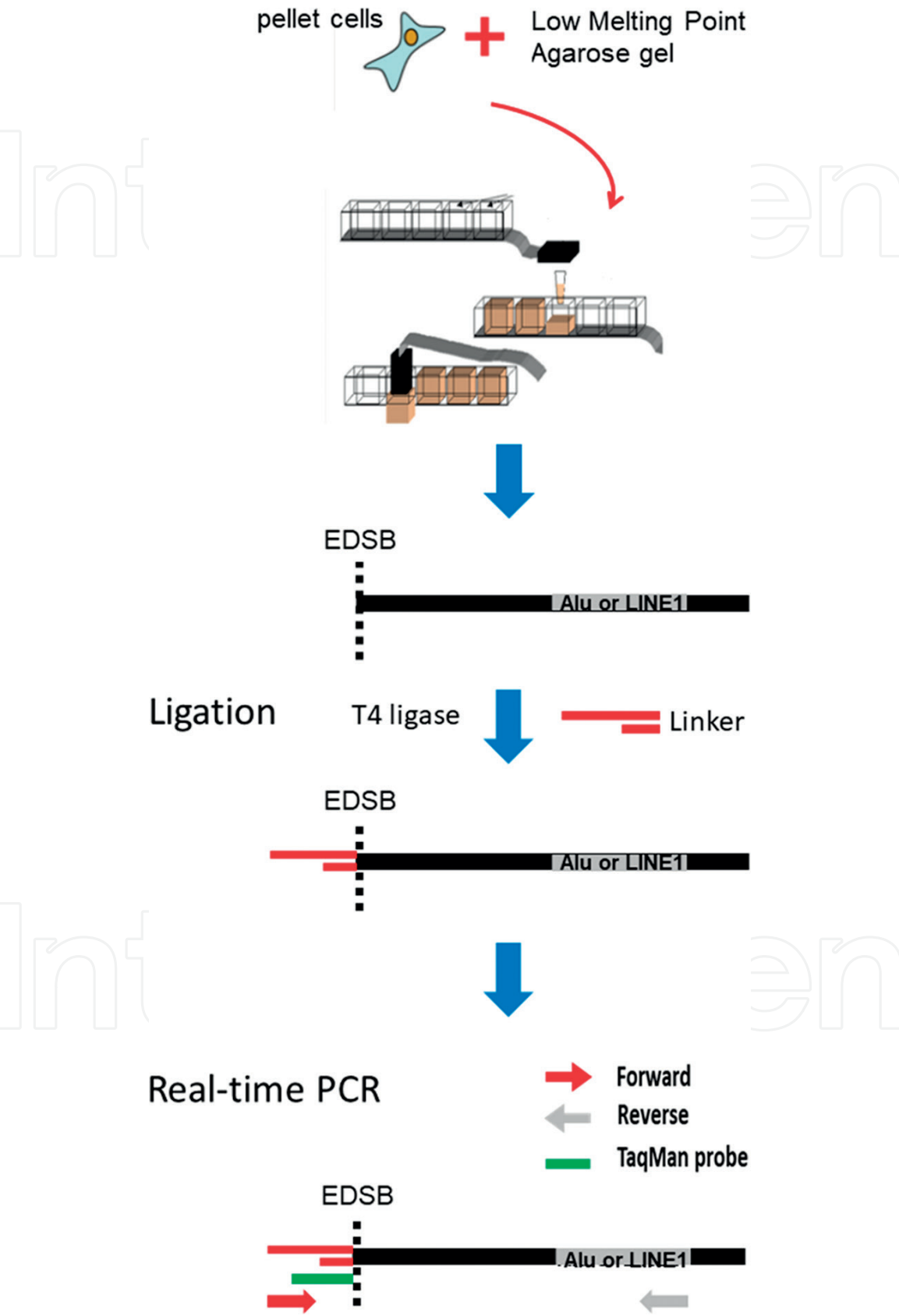
Figure 3. IRS-EDSB-LMPCR diagram demonstrating IRS-EDSB-LMPCR. LMPCR linker ligates to EDSB. The 5' end of the LMPCR linker is the same sequence as the PCR primer. The 3' end of the LMPCR linker is homologous to the Taqman probe. The Taqman probe is used for quantitation of EDSBs by real-time PCR. The IRS primer is a PCR primer with IRS sequences to polymerize numerous locations of the genome [15].
