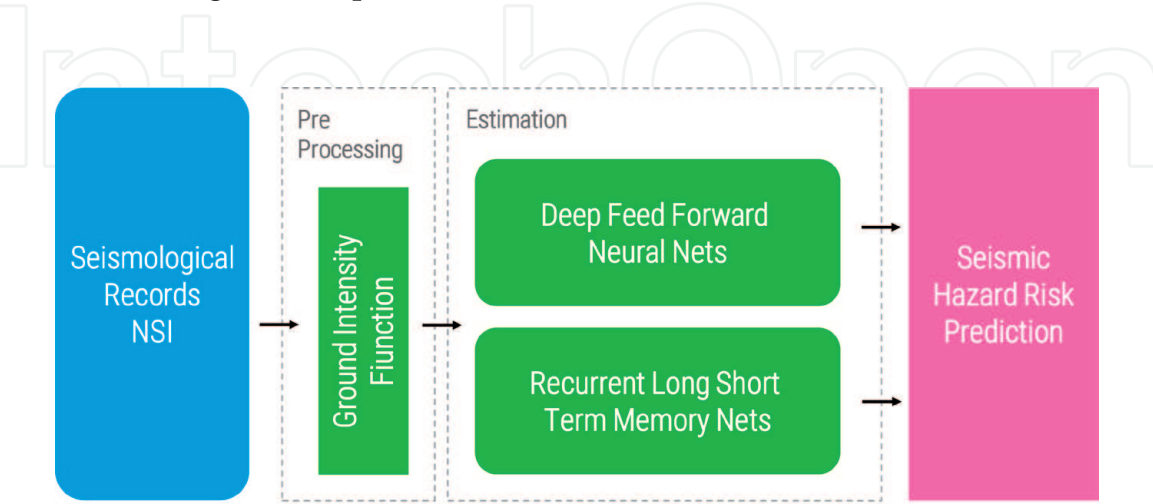
Figure 1. Scheme for the two modular DL neural network framework: data preprocessing and estimation modules. In the data preprocessing module, all data are analyzed and prepared as inputs for the following modules; this considers estimating the daily ground intensity function. The estimation module will receive inputs from the previous model and use DFANN and RNN-LSTM DL to estimate and predict the ground intensity function.
