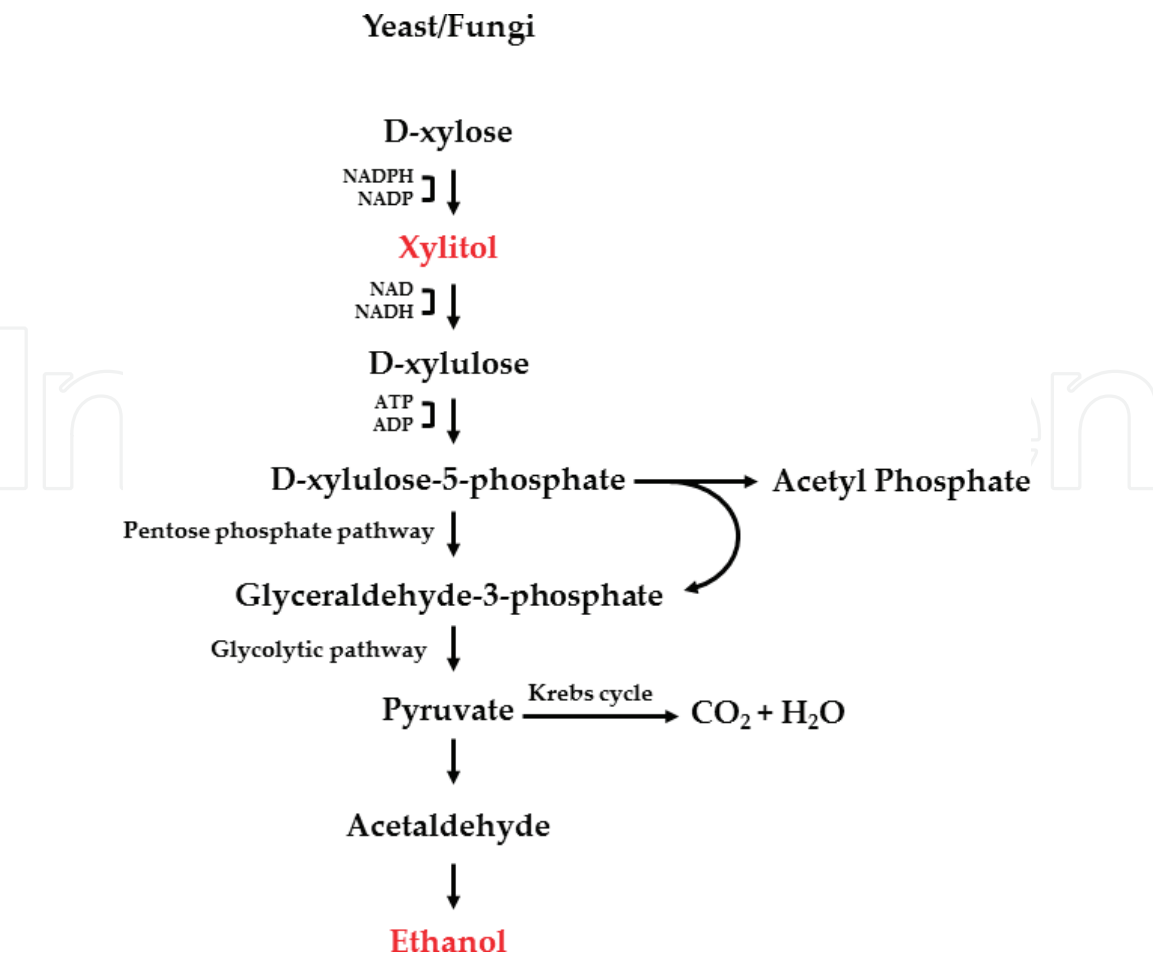
Figure 1. Schematic diagram of D-xylose metabolism.
