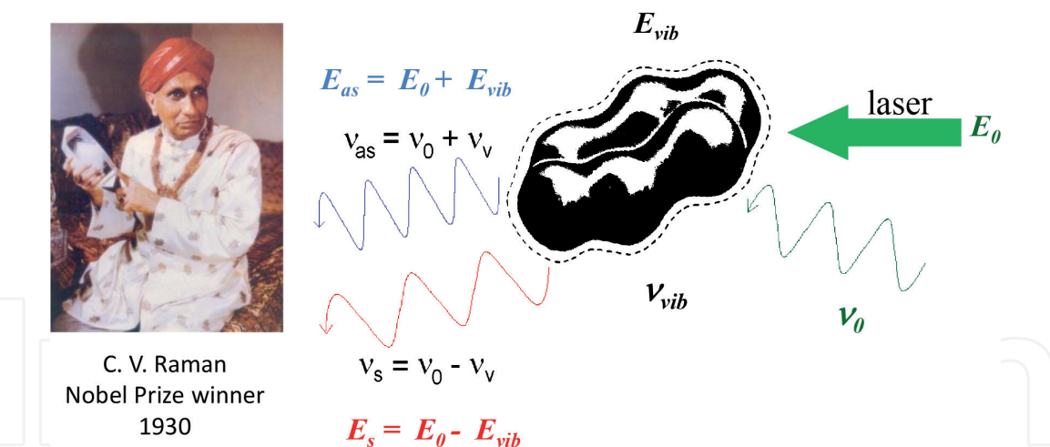
Figure 5. Schematic representation of Raman effect. The Raman scattering was discovered by C. V. Raman and is characterized by inelastic scattering of the incident radiation ( \nu_0 ) with laser energy ( E_0 ). The scattered light has two components: Stokes radiation ( \nu_s ) with lower energy than E_0 ( E_s < E_0 ) and the anti-stoke radiation ( \nu_{as} ) with higher energy than E_0 ( E_{as} > E_0 ).
