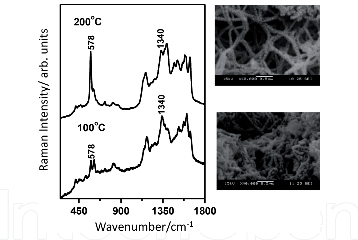
Figure 6. Resonance Raman spectra of PANI-NSA after heating at indicated temperatures and doping with HCl. For comparison the SEM images are also given.
