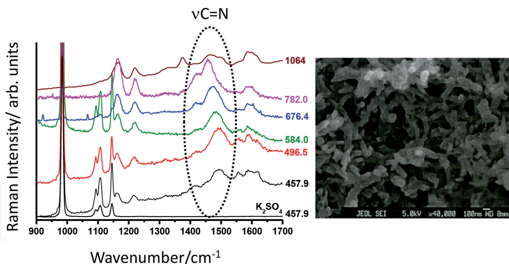
Figure 7. Raman dispersion of PANI nanofibers.
