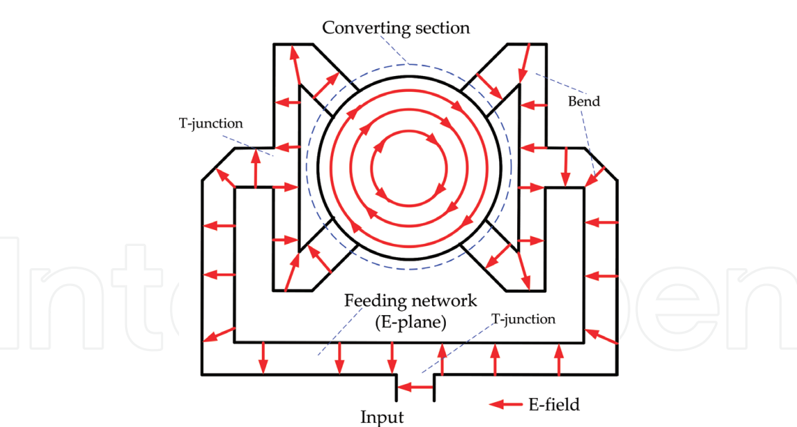
Figure 2. Scheme of a sidewall coupling for a circular waveguide TE_{01} mode transducer, showing the electric field lines, the converting-section (dashed circle) excited in its four sides, and the input feeding network (with E-plane T-junctions and waveguide bends).
