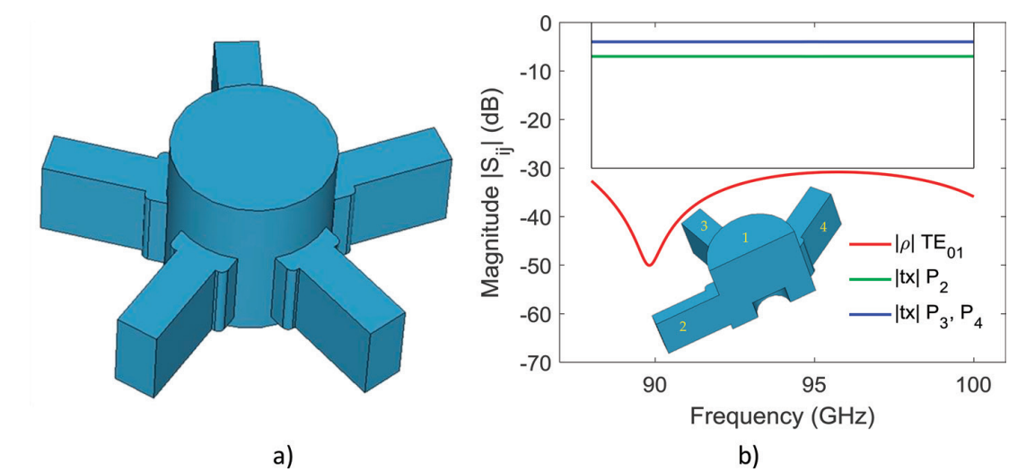
Figure 8. (a) 3D CAD view of the 5-way divider. (b) Simulated response of the reflection coefficient for the circular waveguide TE 01 cir mode, and the transmission to the TE 10 rec rectangular ports (from TE 01 cir ) (only half of the structure); in the inset, a 3D CAD view including the port numbering is shown.
