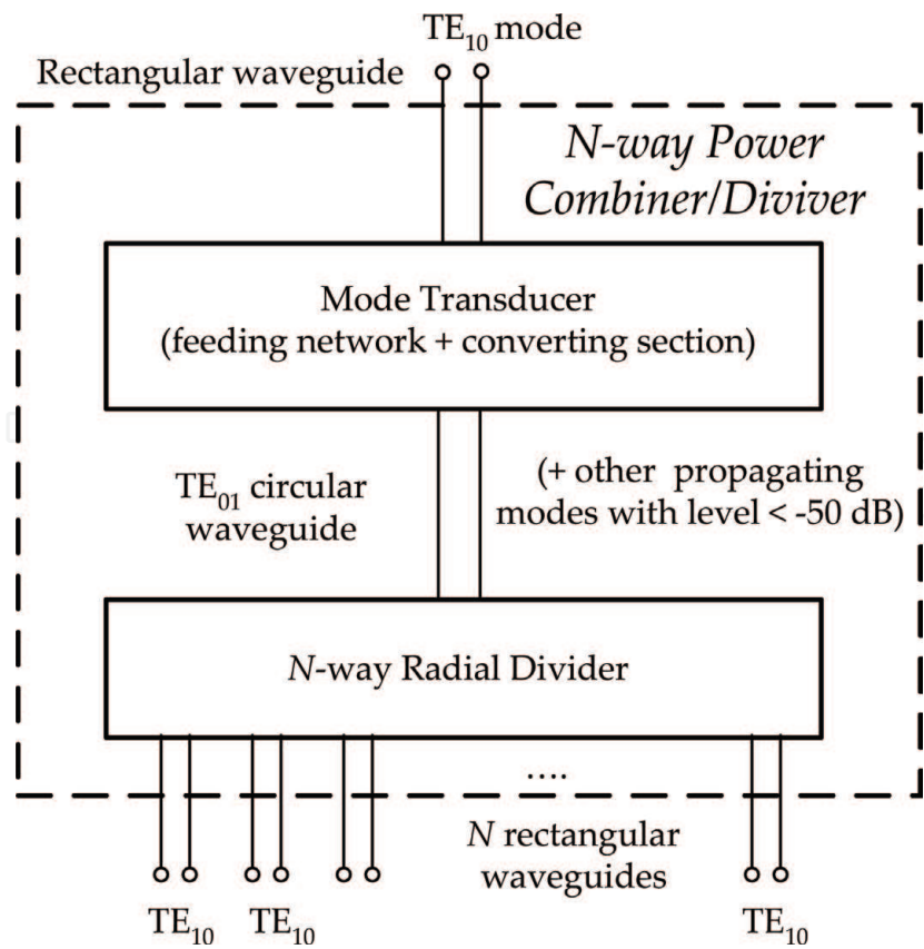
Figure 1. Scheme of the radial power combiner (or divider) made up of (i) the mode transducer between the rectangular waveguide TE_{10} mode and the circular waveguide TE_{01} mode, and (ii) the N-way radial divider (or combiner) dividing the power carried by the circular waveguide TE_{01} mode into N rectangular waveguide TE_{10} modes.
