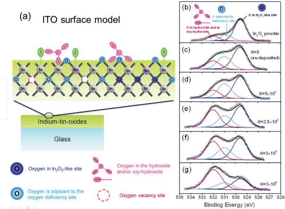
Figure 4. (a) Schematic representation of as-deposited ITO surface composition based on Donley's model [21]. (b) The \text{O}1s XPS spectra of \text{In}_2\text{O}_3 powder and fs laser-treated ITO films with various pulse numbers ( N = 0, 5 \times 10^3, 2.5 \times 10^4, 3 \times 10^5, \text{ and } 3 \times 10^6 , respectively) [11].
