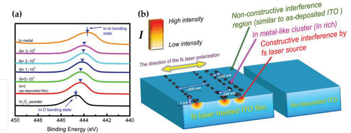
Figure 5. (a) The \text{In } 3d_{5/2} XPS spectra of \text{In}_2\text{O}_3 powder, In metal, and fs laser-treated ITO films with various pulse numbers ( N = 0, 5 \times 10^3, 1 \times 10^5, 3 \times 10^5, \text{ and } 3 \times 10^6 , respectively). (b) A schematic illustration for the formation of self-organized nanodots induced by the constructive interference of fs laser at near-surface region. The dot is composed of In-rich clusters with a height of \sim 5 \text{ nm} as a result of In-O bonding breaking into In-In under local-field enhancement [11].
