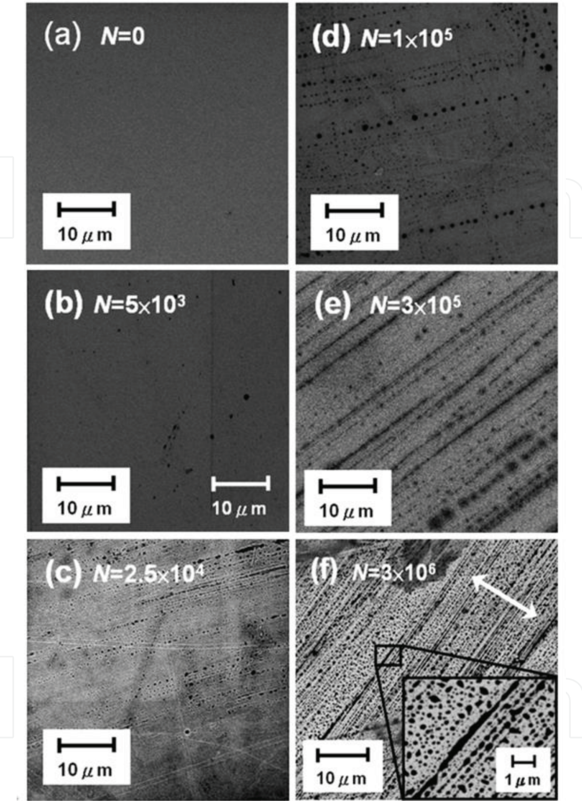
Figure 2. (a–f) SEM images of periodic surface structures induced by 800 nm fs laser pulses at a fluence of 0.1 mJ/cm 2 and with various pulse numbers ( N = 0, 5 \times 10^3, 2.5 \times 10^4, 1 \times 10^5, 3 \times 10^5 , and 3 \times 10^6 , respectively). The black-square inset shows the enlarged surface features at corresponding locations in (f). The arrow indicates the direction of the laser polarization [11].
