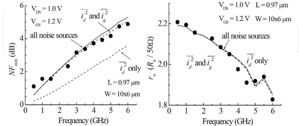
Fig. 3. Impacts of noise sources on NF_{min} and r_n ( R_n normalized to 50\Omega ).
