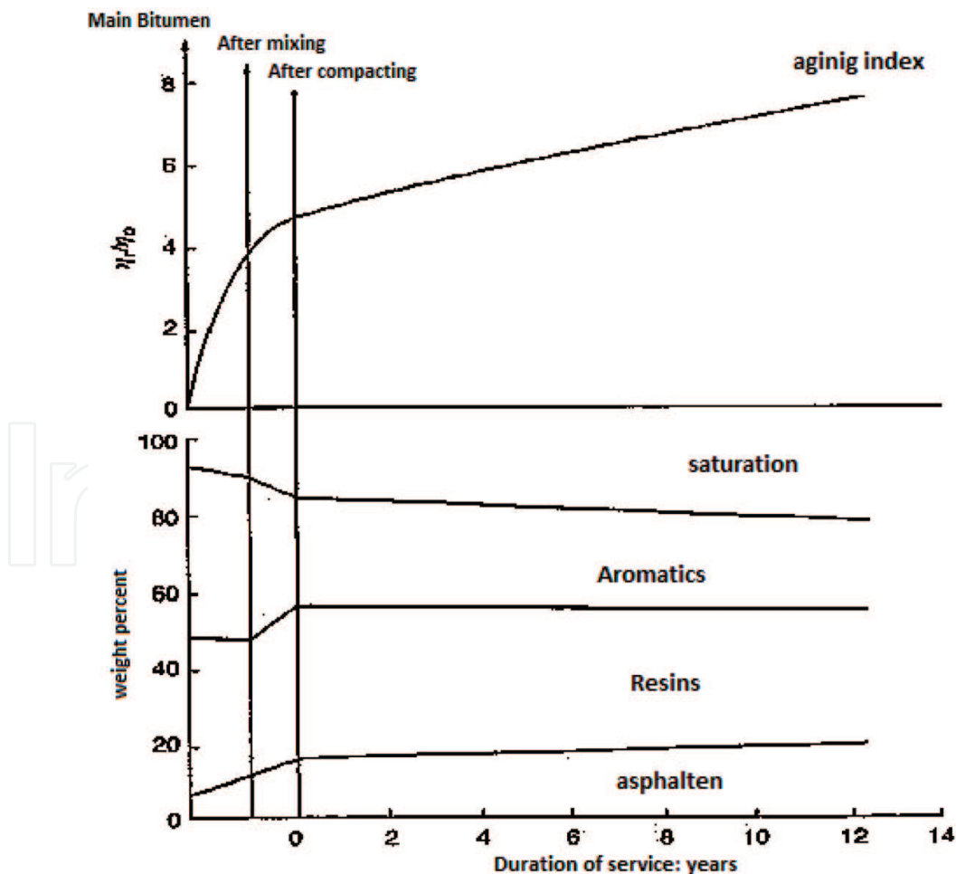
Figure 4. The changes of bitumen components during mixing, diffusing, compacting, and serving.
