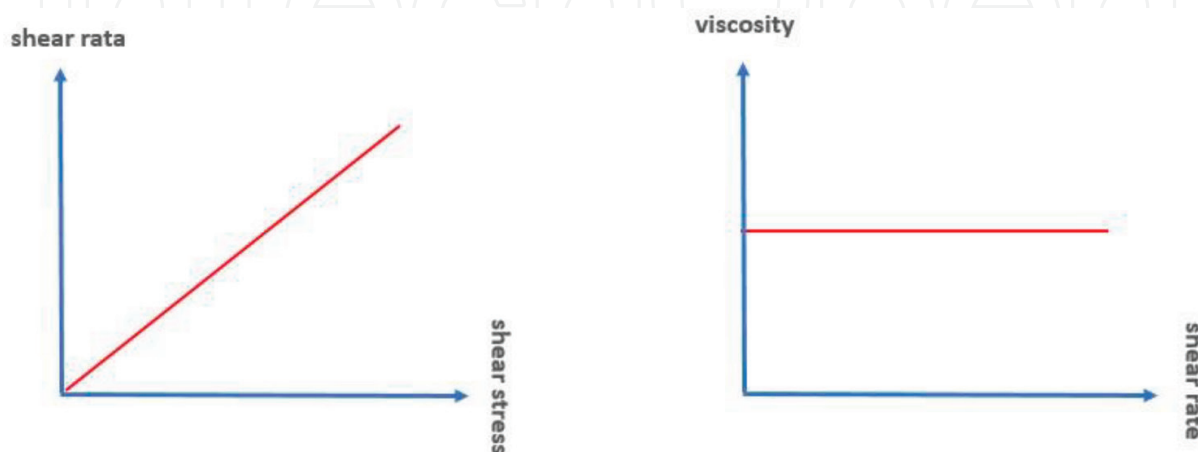
Figure 1. Newtonian behavior [6].
