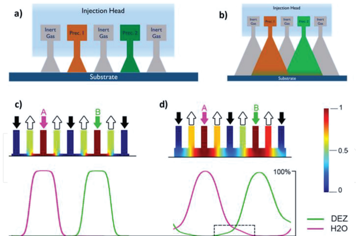
Figure 9. Comparison between SCVD and SALD modes. Scheme of a close-proximity head having two precursor channels and different gaps between head and sample: (a) 150 μm gap, no mixing in the gas phase, (b) 700 μm gap, resulting in precursor mixing above the sample surface, and (c) and (d) show a CFD stationary simulation of the two different modes. A whole representation of the head was used to simulate the behavior of the gases, but only two precursor channels are shown. A cross section of the head with precursor, inert and evacuation channels is shown in which the normalized concentration of the different precursors is given. Below, normalized precursor concentration profiles calculated along the substrate line are shown.
