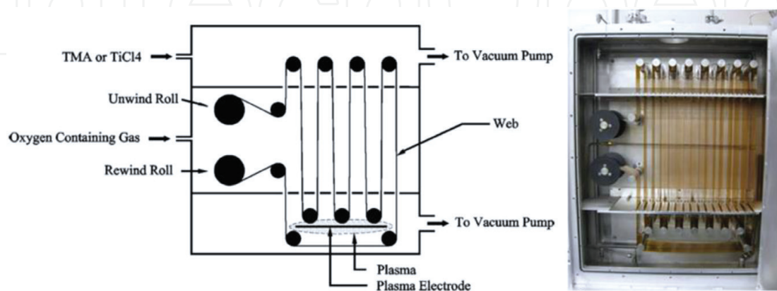
Figure 4. Low-pressure SALD reactor proposed by Lotus Applied Technology. Reproduced from Dickey, E. et al. J. Vac. Sci. Technol. A 30, 021502 (2012), with the permission of the American Vacuum Society.
