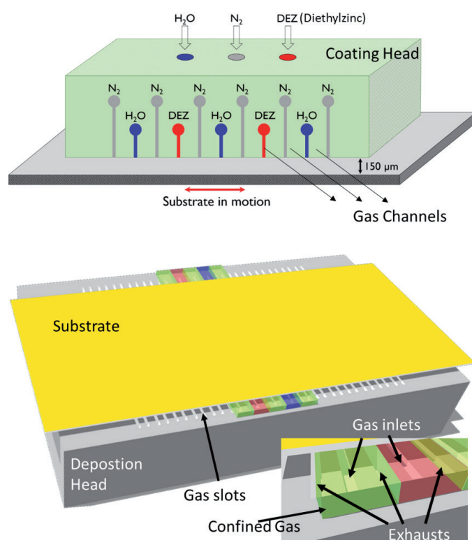
Figure 6. Close-proximity SALD approaches. Left: Schemes of the initial SALD systems reported by Kodak. Right: system developed at the LMGP.
