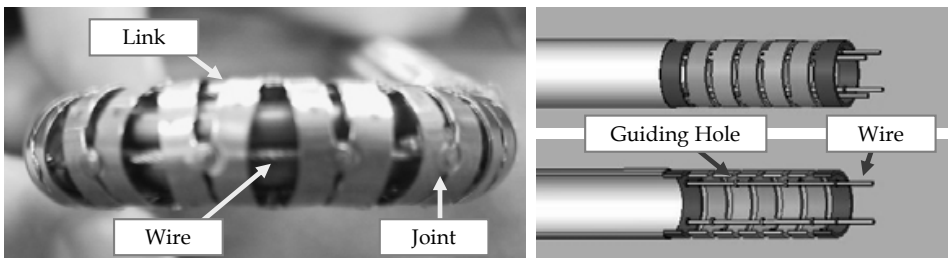
Figure 3. Wire-driven bending mechanism
