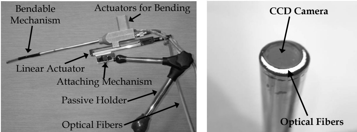
Figure 2. The developed compact laparoscopic assistant robot
