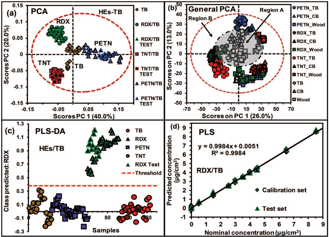
Figure 3. (a) PCA model for QCL detection of HE/TB; (b) general PCA regression model for QCL spectra of HE/substrates. The dotted red closed curve represents a 95% confidence level. (c) Class prediction of HE on TB using PLS-DA; (d) PLS predicted vs. nominal surface concentration of RDX/TB with a correlation coefficient ( R^2 ) of 0.9984.
