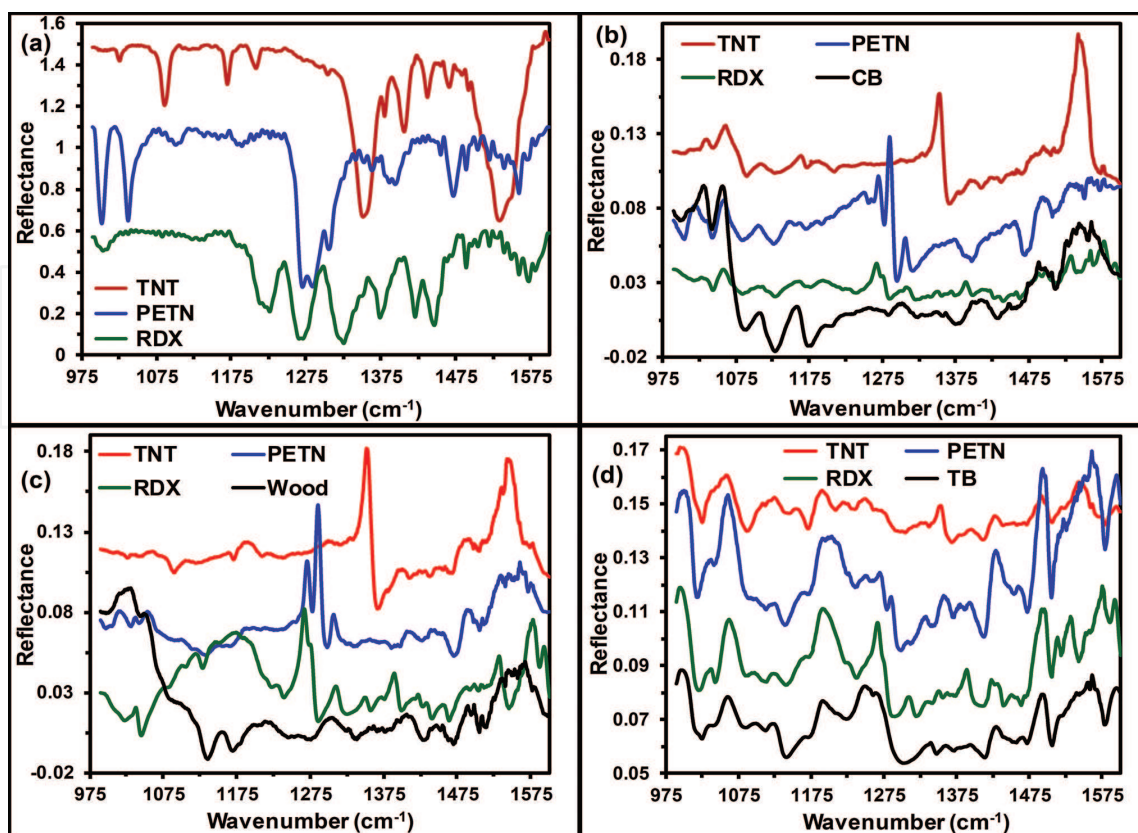
Figure 2. QCL spectra of HEs on substrates studied: (a) Al, reference reflective substrate; (b) CB; (c) wood (W); and (d) TB. Surface concentrations were kept constant at \sim 15\text{ }\mu\text{g}/\text{cm}^2 for comparison purposes. Reflectance spectra of matte substrates are included to denote the extent of spectroscopic intrusion.
