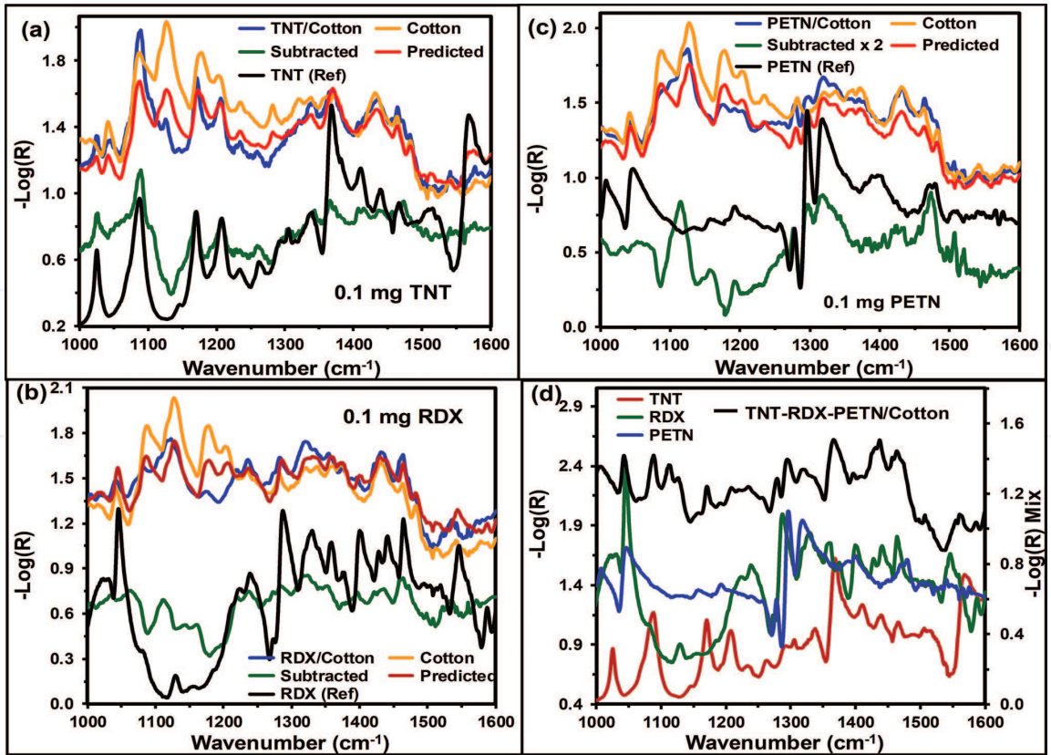
Figure 6. (a–c) Spectra of ~0.1 mg of HE/cotton (blue); predicted spectra from Eq. (5) (red traces); cotton spectra (orange); subtraction of the cotton spectra from HE/cotton spectra calculated using Eq. (4) (green); reference HE spectra (black); (d) comparison of reference spectra of HE and a spectrum for the quaternary mixture: TNT-RDX-PETN/cotton.
