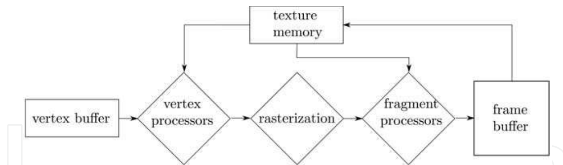
Fig. 3. The graphics rendering pipeline. Geometric primitives are loaded into the vertex buffer and transformed by multiple vertex processors in parallel. The rasterization samples the geometry into pixel positions such that multiple fragment processors can assign colors that are recorded in the frame buffer for the final image.
