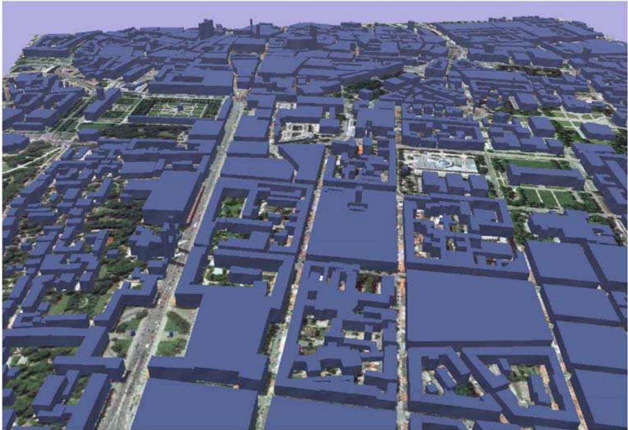
Fig. 1. Typical propagation environment with 2.5 dimensional building structures. The underlying satellite image provides geographical reference.
