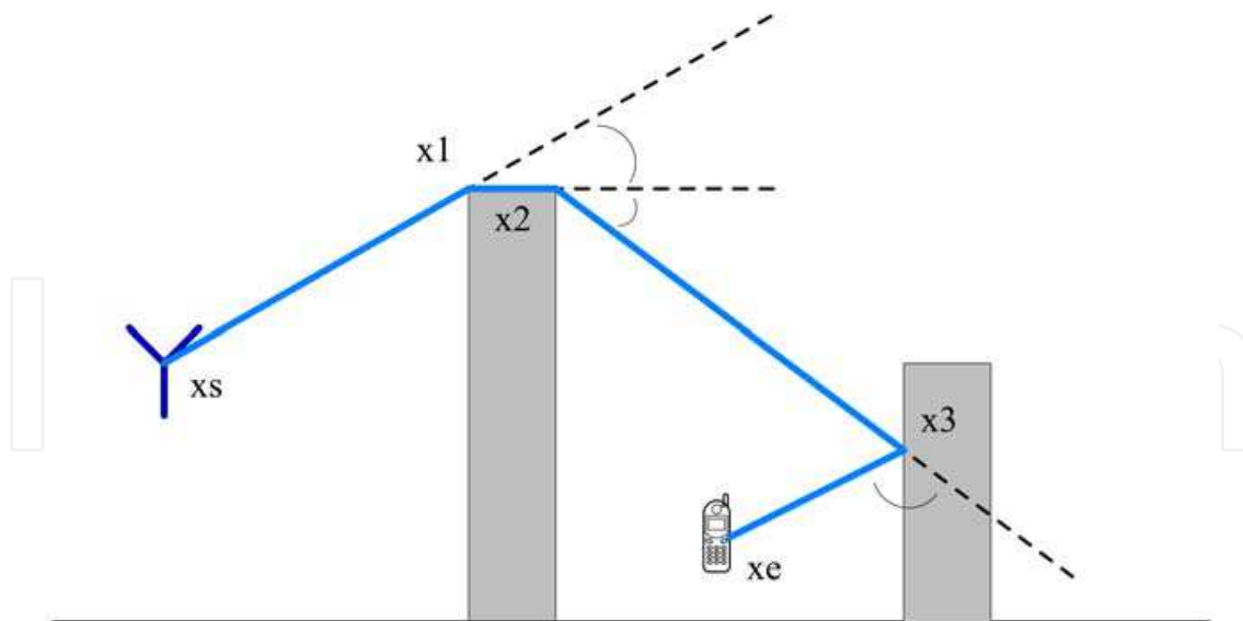
Fig. 4. Example propagation path (side profile). A ray is emanating from the radiation source, diffracted at the rooftop of the first building and reflected the second building into the street: x_s \rightsquigarrow x_1 \rightsquigarrow x_2 \rightsquigarrow x_3 \rightsquigarrow x_e .
