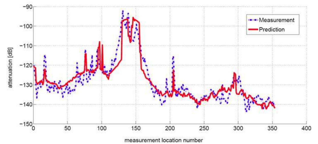
Fig. 12. Comparison between measured and predicted pathloss along route METRO201 in COST 231 Munich.
