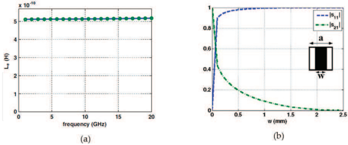
Figure 5. Frequency variations in equivalent inductance (a) and the variation in S parameters versus the width of strip for 10 GHz (b) [7].
