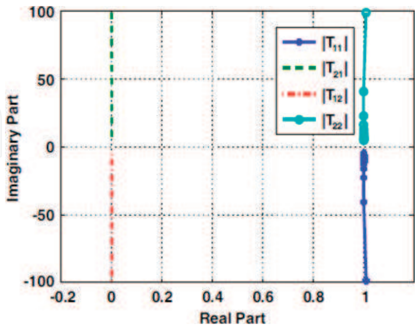
Figure 15. The locus of scattering transfer parameters for the square perforated metal plate [7].
