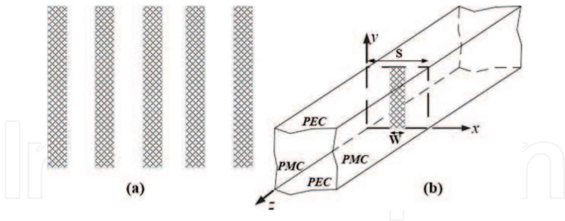
Figure 3. Metal strip grating (a), a unit cell of the structure with suitable boundary conditions in peripheral (parallel polarization) (b) [7].
