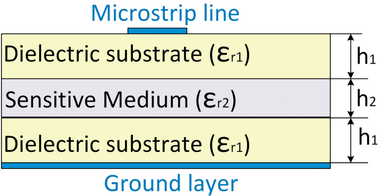
Figure 6. Microstrip line on tri-layered substrate.
