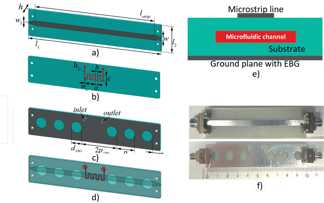
Figure 13. Microfluidic EBG sensor: (a) top layer, (b) substrate with embedded channel, (c) bottom layer with defected EBG, (d) 3D view, (e) cross section, and (f) top and bottom side of the fabricated sensor [14].
