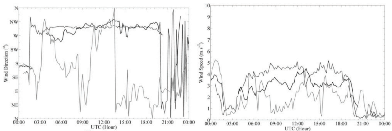
Figure 5. March 06, 2011. Left panel is the mean wind direction and right panel is the wind speed evolution in the ASL, ABL layers, and FA. In the left panel, black solid line represents 10 min average wind direction measured by sonic anemometer 4 m height, the black dash line represents the ABL wind speed at 55 m measured by the sodar, and the gray line represent the 165 m measured by the sodar. In the right panel, black solid line represents 10 min average wind speed measured by sonic anemometer 4 m height, the black dash line represents the ABL wind speed at 55 m measured by the sodar, and the gray line represents the 165 m measured by the sodar in the FA.
