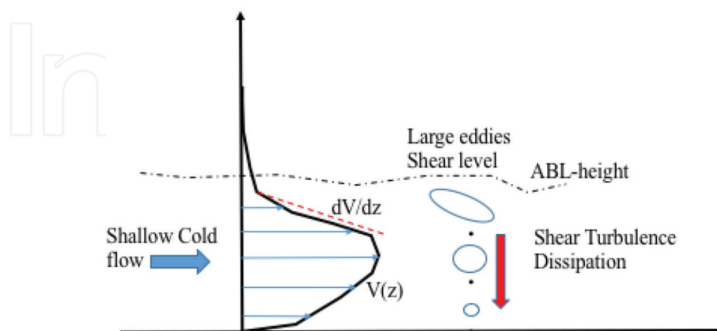
Figure 15. Conceptual scheme describing the mechanism for shear induced turbulence in the presence of a shallow cold flow. Upper ABL level illustrates wind speed shear that breaks down propagating and dissipating toward the surface. These localized large eddies impact the optical turbulence signature of LAS.
