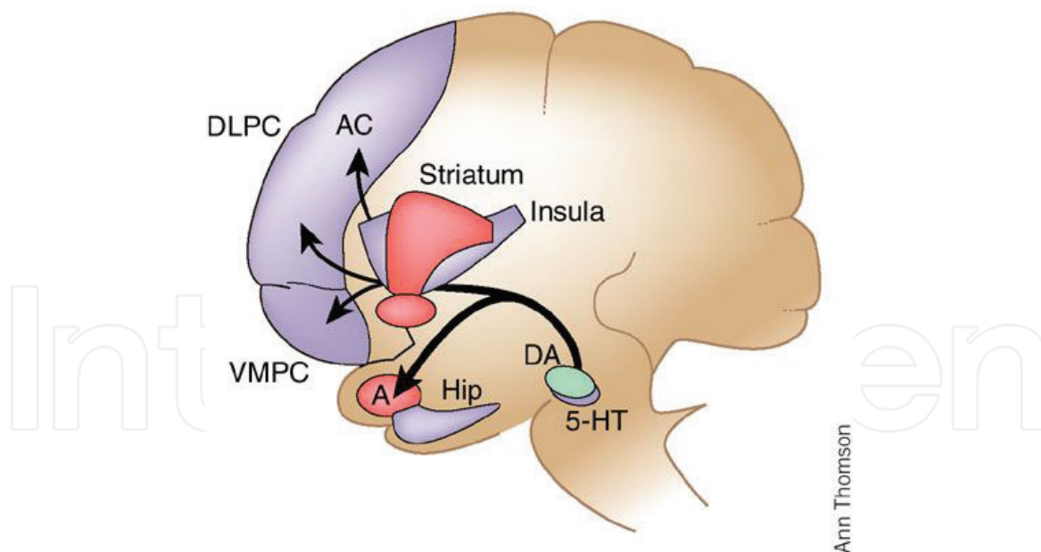
Figure 1. Diagram from key structures involved in the impulsive (red) and reflective system (blue). A: amygdala, VMPC: ventromedial prefrontal cortex, AC: anterior cingulate, DLPFC: dorsolateral prefrontal cortex, hip: hippocampus, DA: dopamine, and 5-HT: serotonin. Extracted from Ref. [33].
