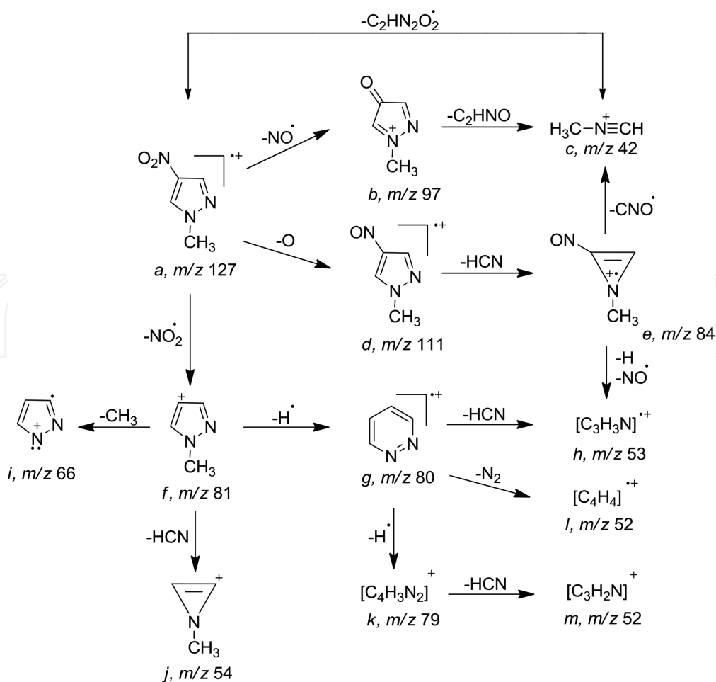
Figure 18. Fragmentation of 1-methyl-4-nitropyrrole 29.
