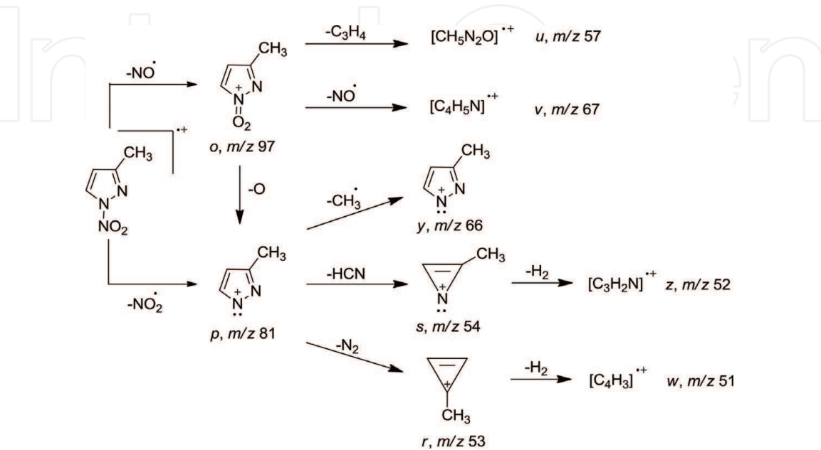
Figure 15. Fragmentation of 1-nitro-3-methylpyrazole 25.
