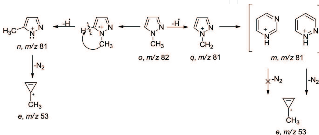
Figure 10. Principal mass fragmentation of compound 10 .
