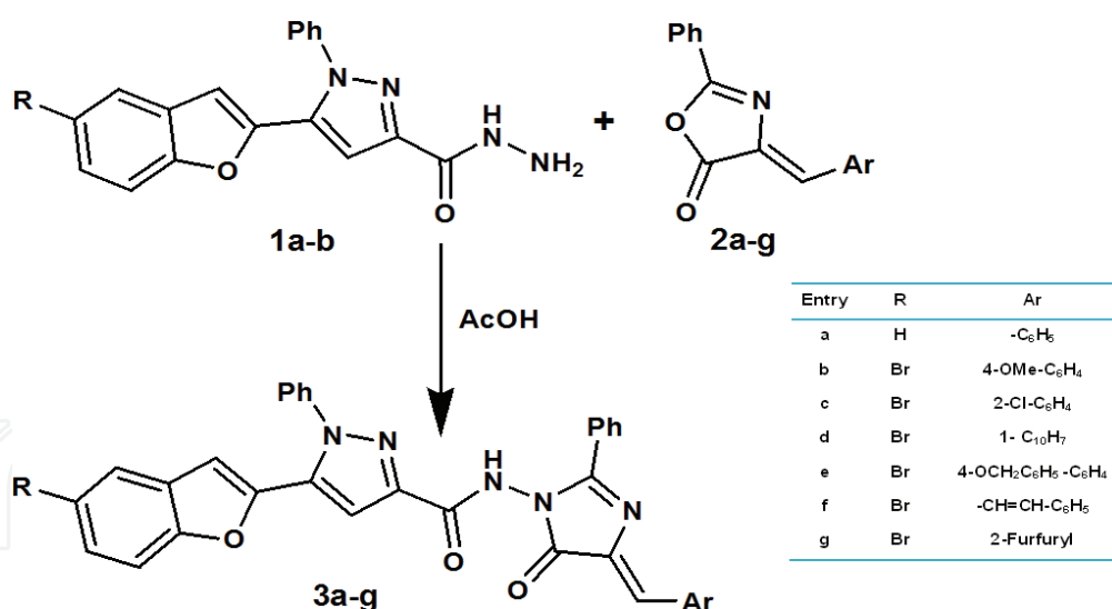
Figure 2. Reaction scheme for 5-oxo-imidazoline derivatives.
