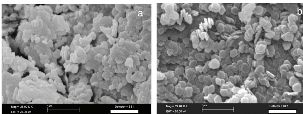
Figure 2. Scanning electron micrographs of (a) kaolinite and (b) gibbsite samples.
