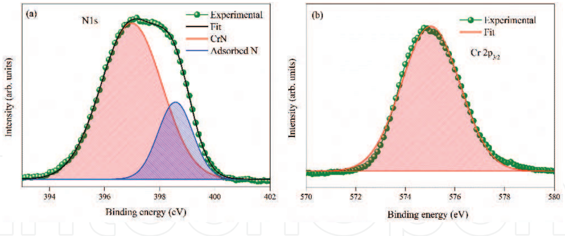
Figure 3. (a) XPS spectra of N1s, and (b) XPS spectra of Cr 2 p 3/2 . (Adapted from Mohd. Arif et al., with permission from Elsevier. Copyright 2018) [23].
