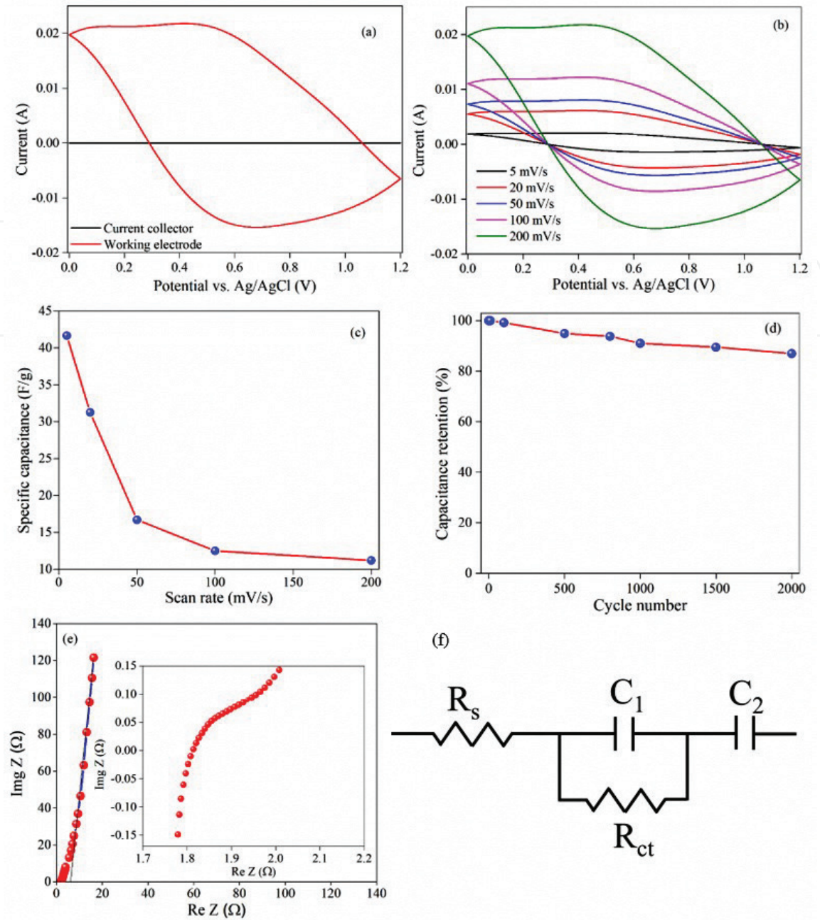
Figure 5. (a) CV curve of CrN working electrode and steel current collector at 200 mV/s, (b) CV curve of CrN working electrode at different scan rates, (c) specific capacitance vs. scan rate graph, (d) capacitive retention curve of CrN thin film working electrode, (e) Nyquist plot (inset shows the enlarged Nyquist plot at the high frequency region), and (f) corresponding equivalent circuit model. (Adapted from Mohd. Arif et al., with permission from Elsevier. Copyright 2018) [23.]
