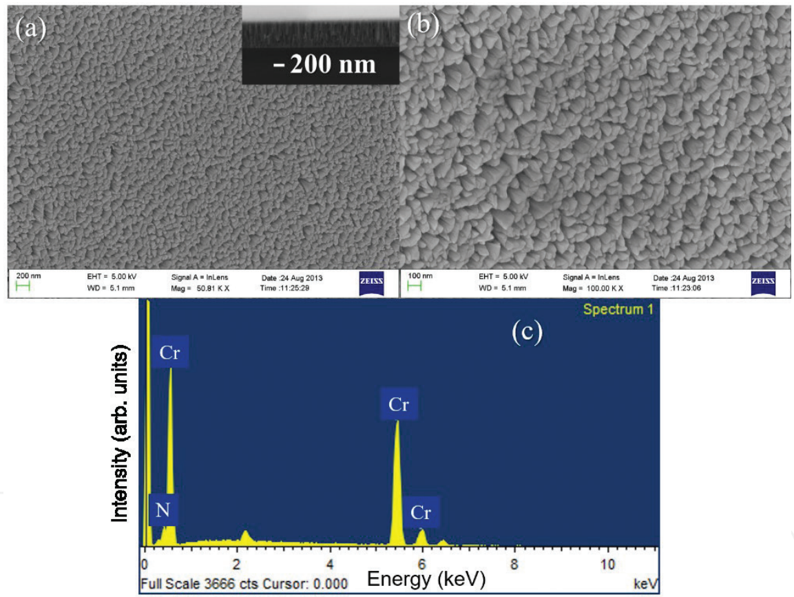
Figure 4. (a and b) FE-SEM images of CrN thin film at different scales, 200 and 100 nm scales, and (c) EDS spectrum of CrN thin film. (Adapted from Mohd. Arif et al., with permission from Elsevier. Copyright 2018) [23].
