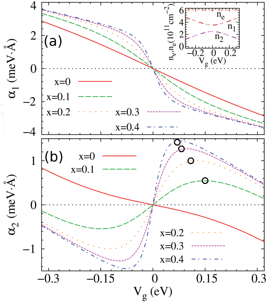
Figure 7. Intraband Rashba \alpha_1 (a) and \alpha_2 (b) couplings as a function of V_g in GaAs/Al 0.3 Ga 0.7 As wells for several Al contents x of a central barrier Al x Ga 1- x As. In (a), the inset shows the gate dependence of electron occupations n_1 , n_2 , and n_e = n_1 + n_2 . In (b), the black circles indicate where \alpha_2 exhibits the maximum, from Wang et al. [40].
