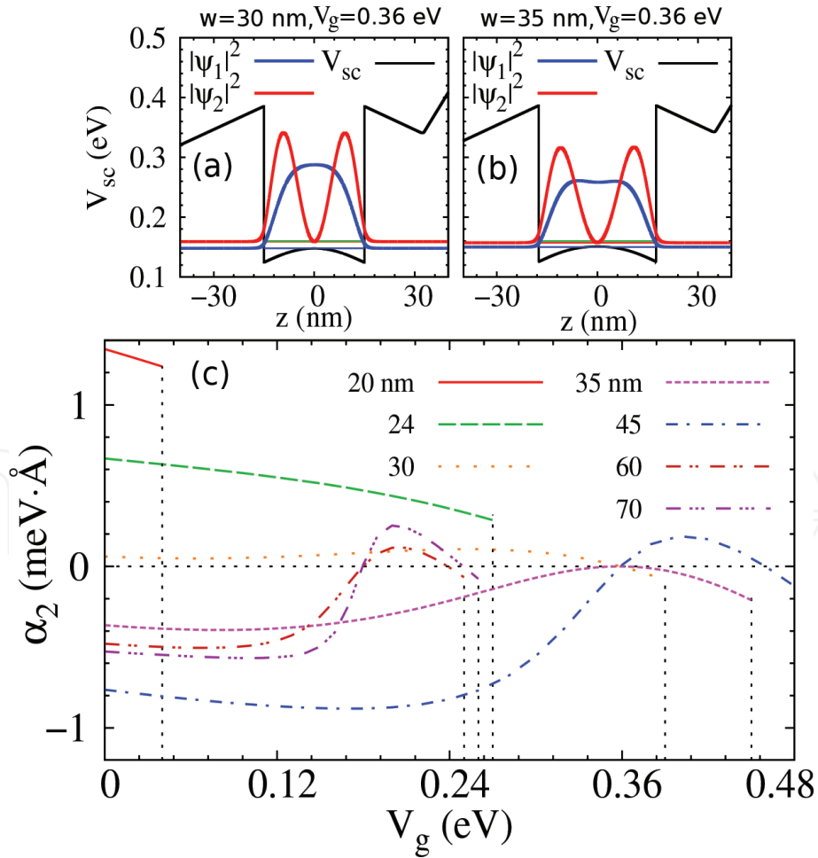
Figure 6. Confining potential V_{sc} and wave function profiles \psi_v in GaAs wells at V_g \sim 0.36 eV (symmetric geometry), for a 30-nm well (a) and a 35-nm well (b). the horizontal lines inside the wells indicate the two-subband energy levels and the Fermi level (c). the dependence of intrasubband Rashba \alpha_2 of the second subband on V_g , for a set of wells of w = 20, 24, 30, 35, 45, 60 , and 70 nm. The vertical dashed lines mark regions of one- and two-band occupations. The temperature is held fixed at 0.3 K, from Wang et al. [32].
