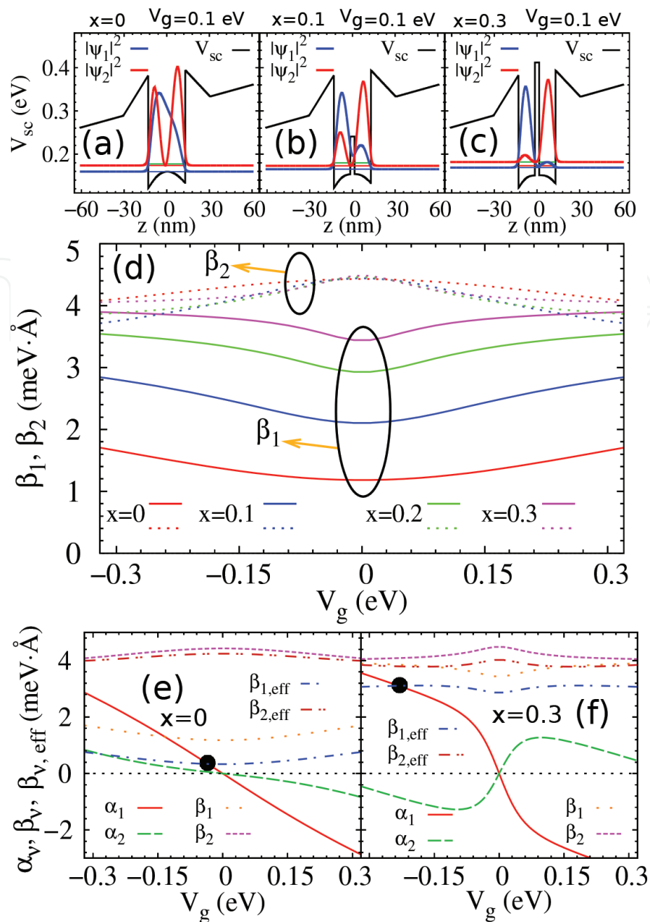
Figure 8. (a)–(c) Self-consistent potential V_{sc} and wave function profiles \psi_v for a GaAs/Al 0.3 Ga 0.7 As well with Al x Ga 1-x As as a central barrier, with x = 0 (a), 0.1 (b), and 0.3 (c). We consider V_g = 0.1 eV. The horizontal lines inside the well indicate the two-subband energy levels and the Fermi level. (d) Intrasubband Dresselhaus terms \beta_v as a function of V_g , for several values of x with x = 0, 0.1, 0.2, 0.3 . (e) and (f) Gate dependence of SO strengths ( \alpha_v, \beta_v, \beta_{v,eff} ) for x = 0 and x = 0.3 , respectively. The black points indicate the PSH symmetry points (i.e., \alpha_v = \pm\beta_{v,eff} ), from Wang et al. [40].
