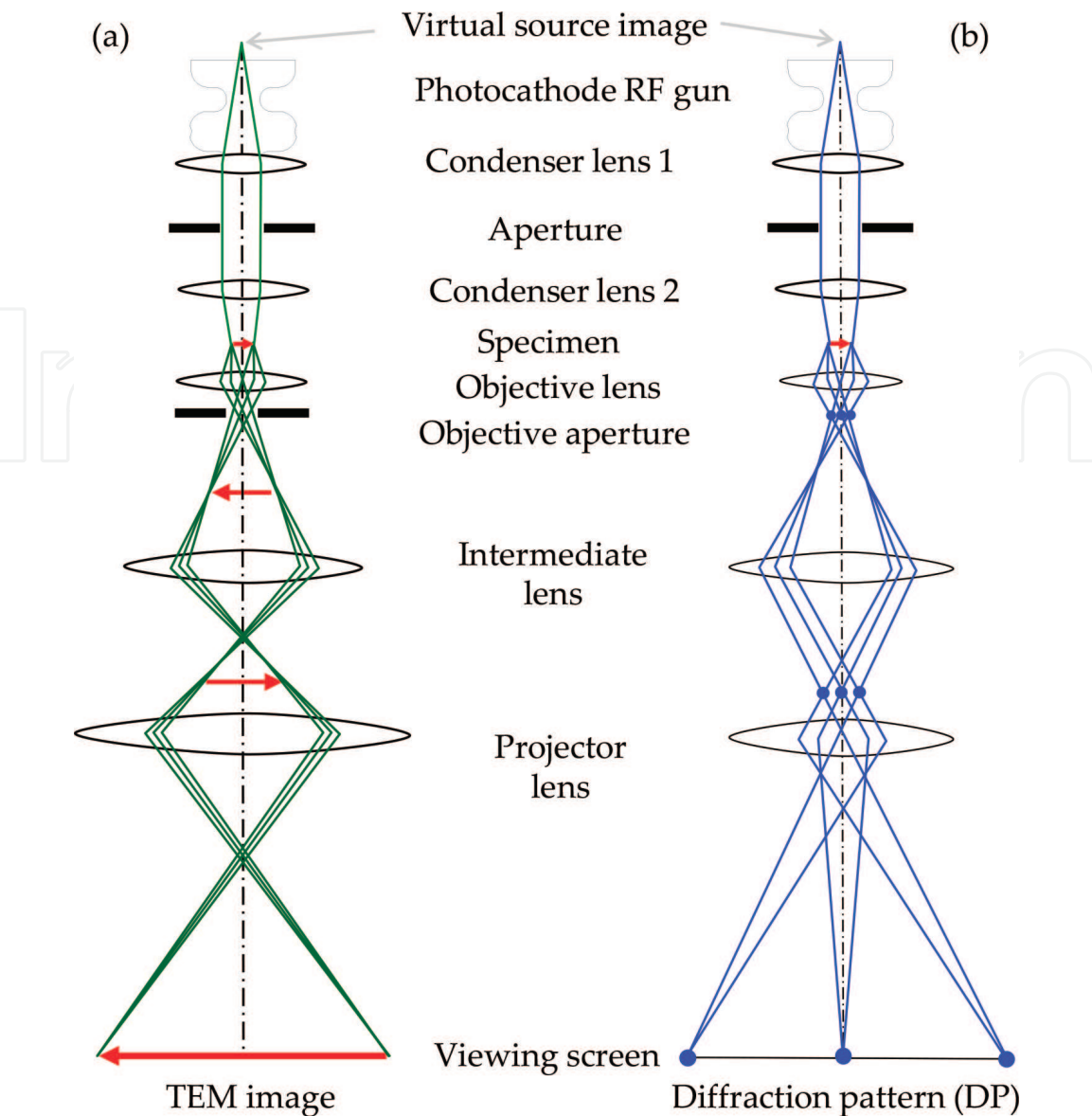
Figure 5. Two basic operations of the UEM imaging system: (a) imaging mode: Projection of a TEM image onto the viewing screen and (b) diffraction mode: Projection of diffraction patterns (DPs) onto the screen.
