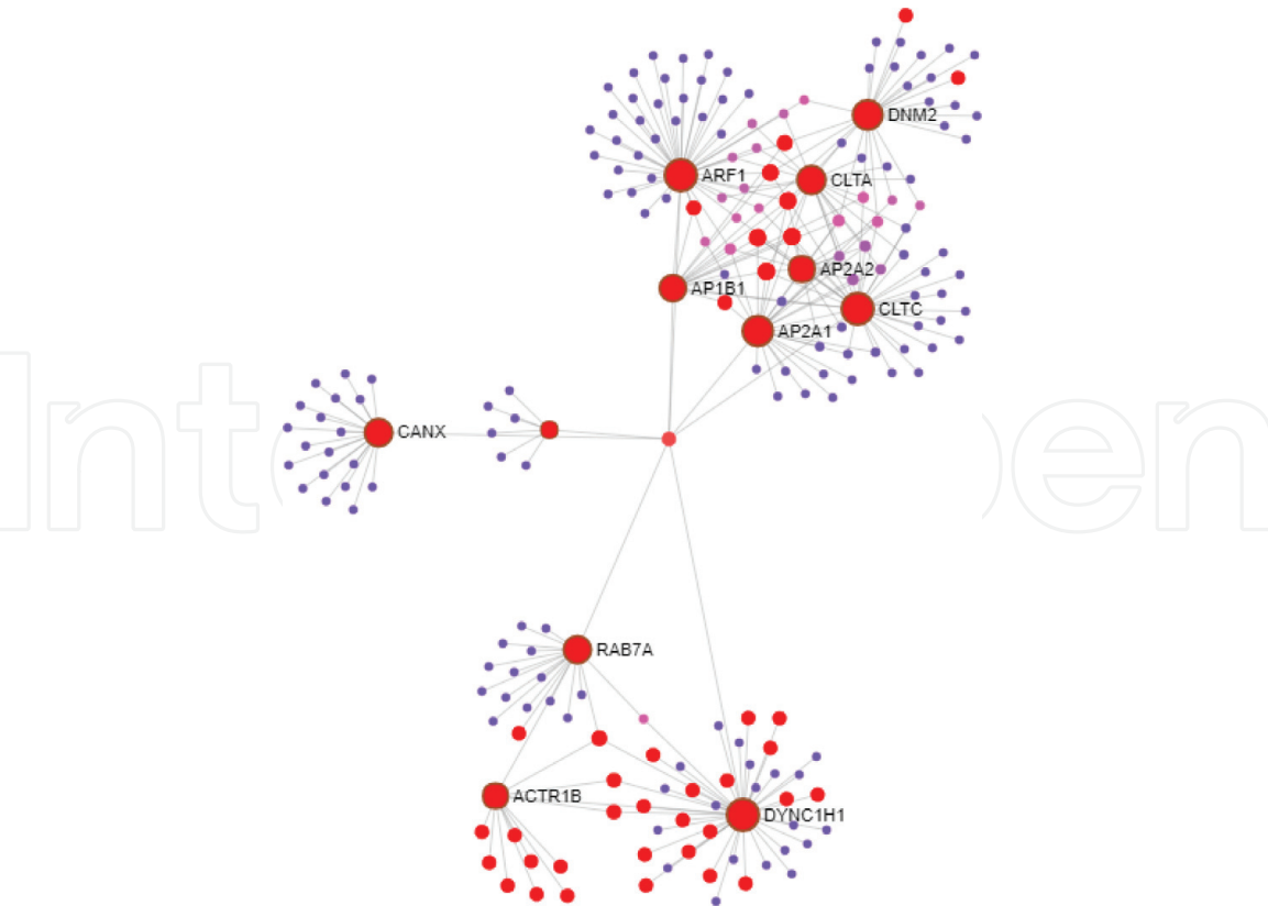
Figure 4. An overview of protein–protein interaction network of a set of proteins, identified in rainbow trout proteome profiling, related to antigen processing and presentation of exogenous peptide antigen via MHCII. Protein–protein interaction network was constructed using NetworkAnalyst software [75]. Highlighted red nodes represent the input protein-related antigen processing and presentation of exogenous peptide antigen via MHCII pathway (Reactome database). Other nodes represent other protein interactions within the same pathway (red nodes) or related to other pathways (other colors).
