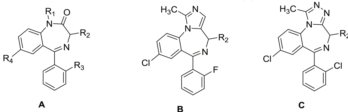
Figure 4. General structure of various BZDs: (A) 5-Aryl-1,4-benzodiazepine; (B) midazolam , a diazobenzodiazepine; and (C) triazolam , a triazolobenzodiazepine [11].
