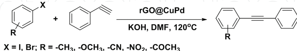
Scheme 14. rGO-CuPd catalyzed Sonogashira couplings of various aryl halides and phenyl acetylene (from Diyarbakir et al. [76]).
