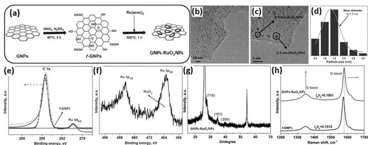
Figure 3. (a) Schematic illustration for the preparation of GNP-RuO 2 NPs, (b and c) TEM images, (d) RuO 2 particle distribution, (e and f) XPS, (g) XRD patterns, and (h) Raman spectra of GNP-RuO 2 NPs (from Gopiraman et al. [32]).
