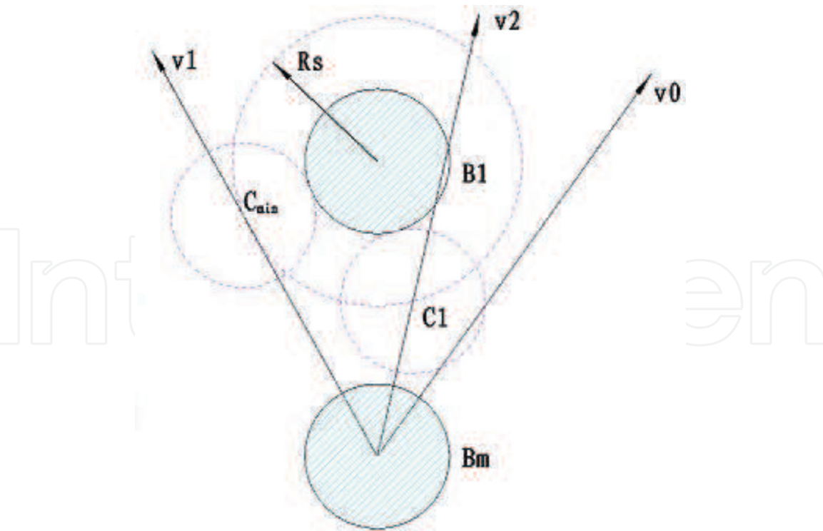
Figure 6. The diagram of single particle collisions.
