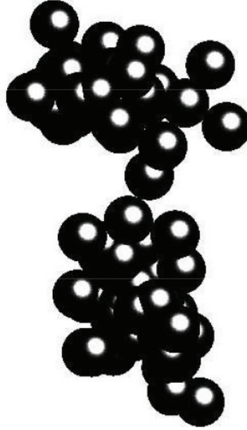
Figure 4. The collision of single particles and single particle.
