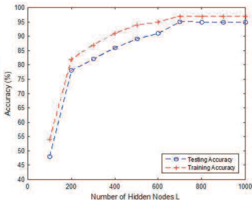
Figure 6. The number of hidden layer nodes L determination with L = 700 .
