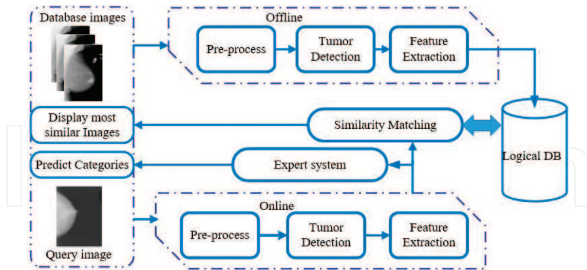
Figure 1. Dataflow diagram of the integrated decision support system (DSS).
