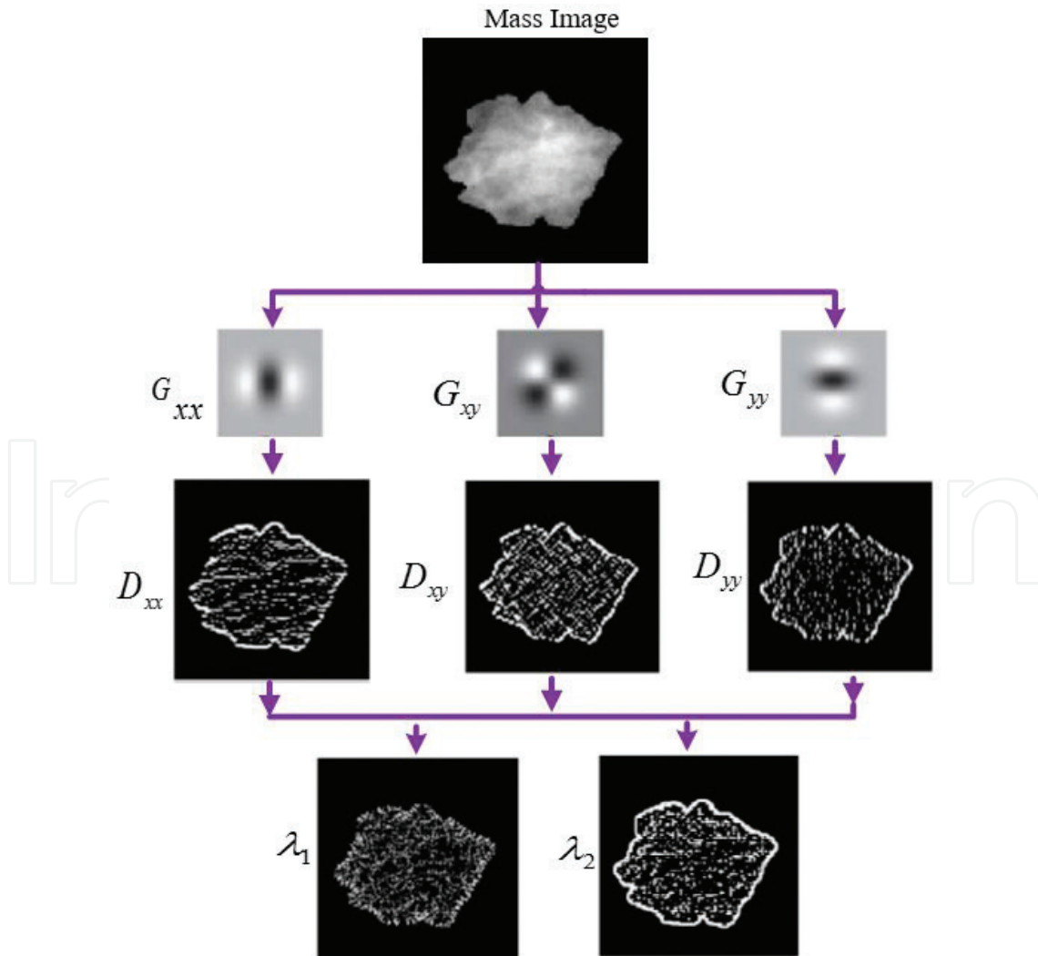
Figure 4. Computation of eigenvalues of the hessian matrix for an ROI as breast mass.
