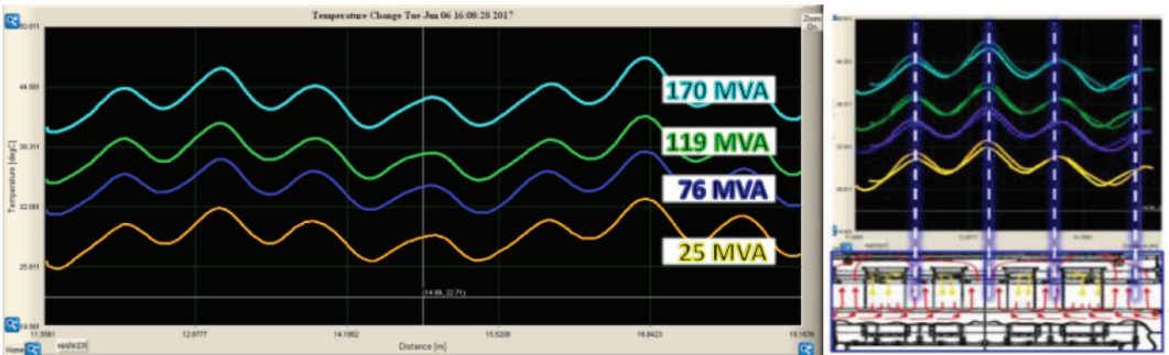
Figure 20. At left, temperature profiles at different loading intensities. At right, temperature profile line-ups with the air duct locations. Courtesy of Oz Optics, Ltd.
