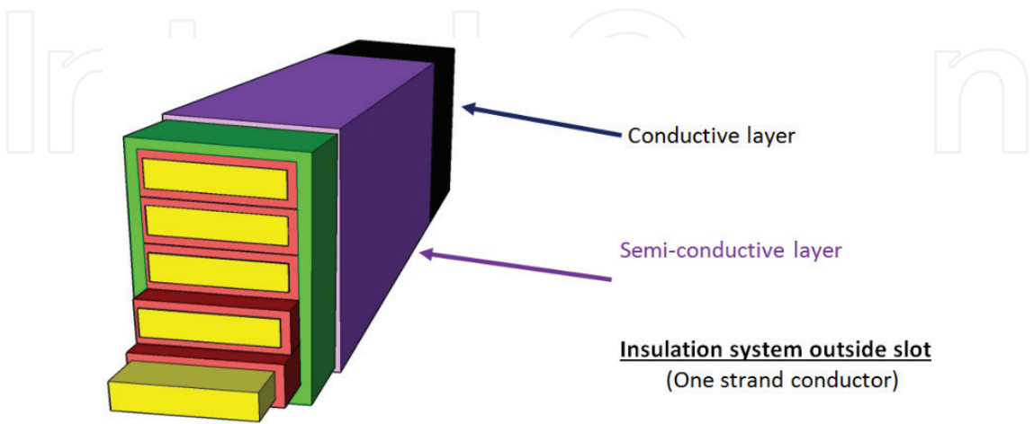
Figure 3. Conceptual depiction of the various insulation subdivisions. Courtesy of QPS Photonics.
