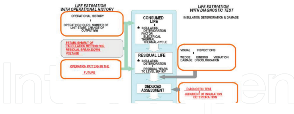
Figure 24. Damage model that allows residual life predictions.
