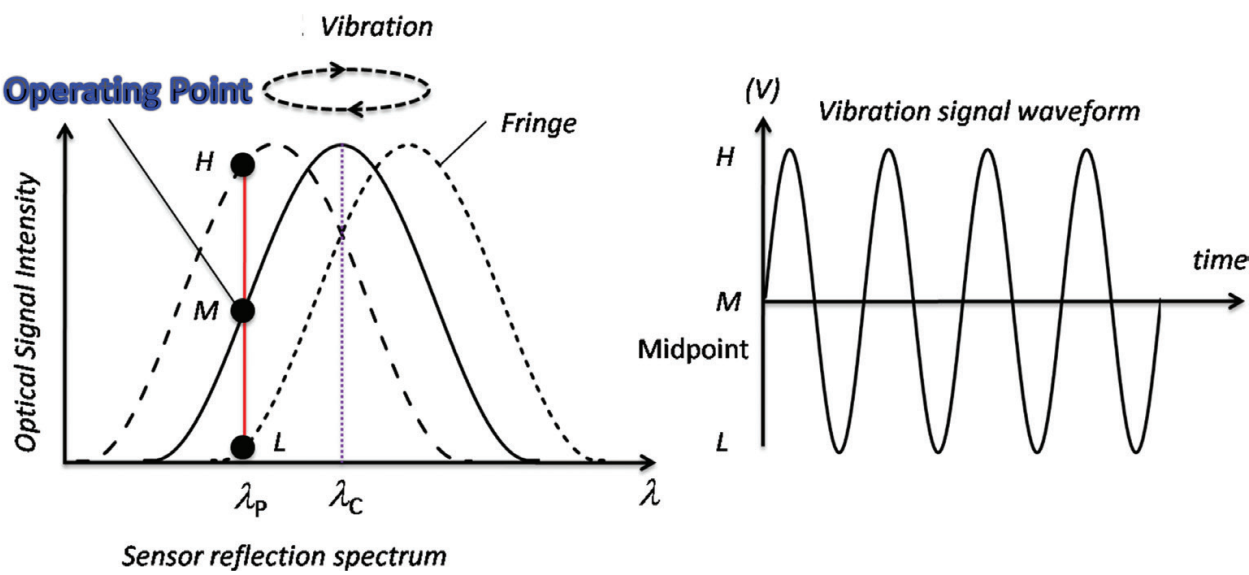
Figure 8. The principle of optical fiber sensing.
