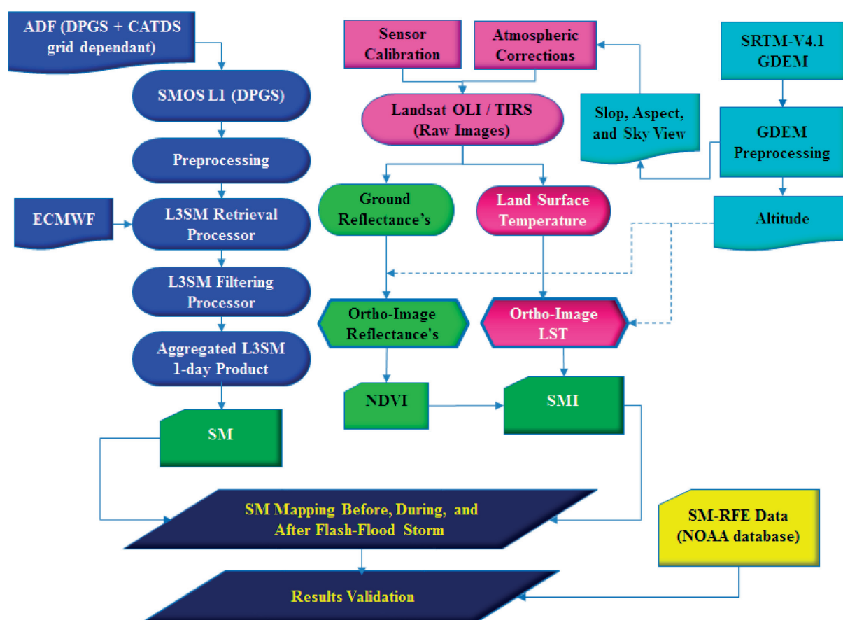
Figure 2. Methodology flowchart.
