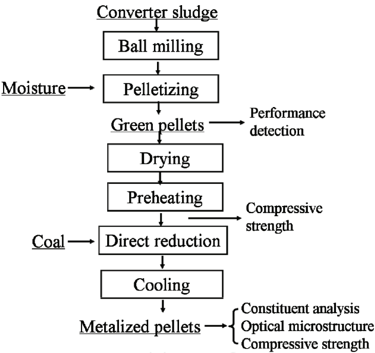
Figure 10. Flow diagram of direct reduction experiment.
