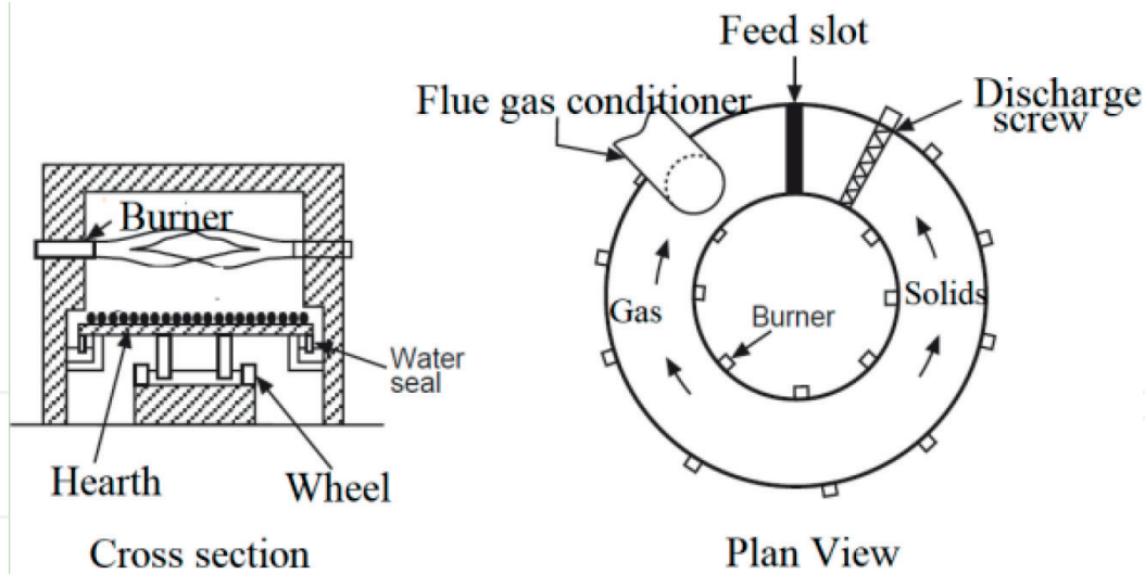
Figure 4. Cross section and plan view of the rotary hearth furnace [30].
