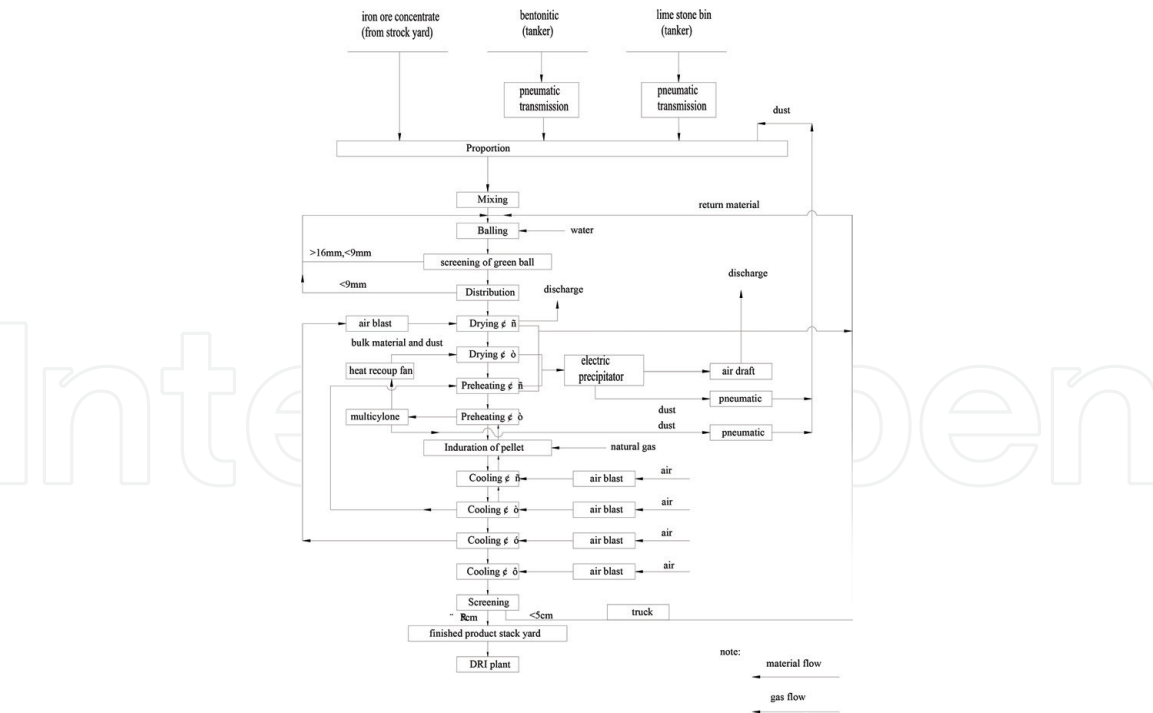
Figure 1. Process flow chart of grate-kiln pelletizing plant.
