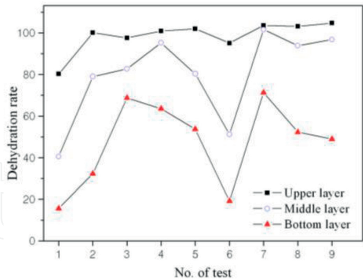
Figure 9. Dehydration rate of dried pellets.
