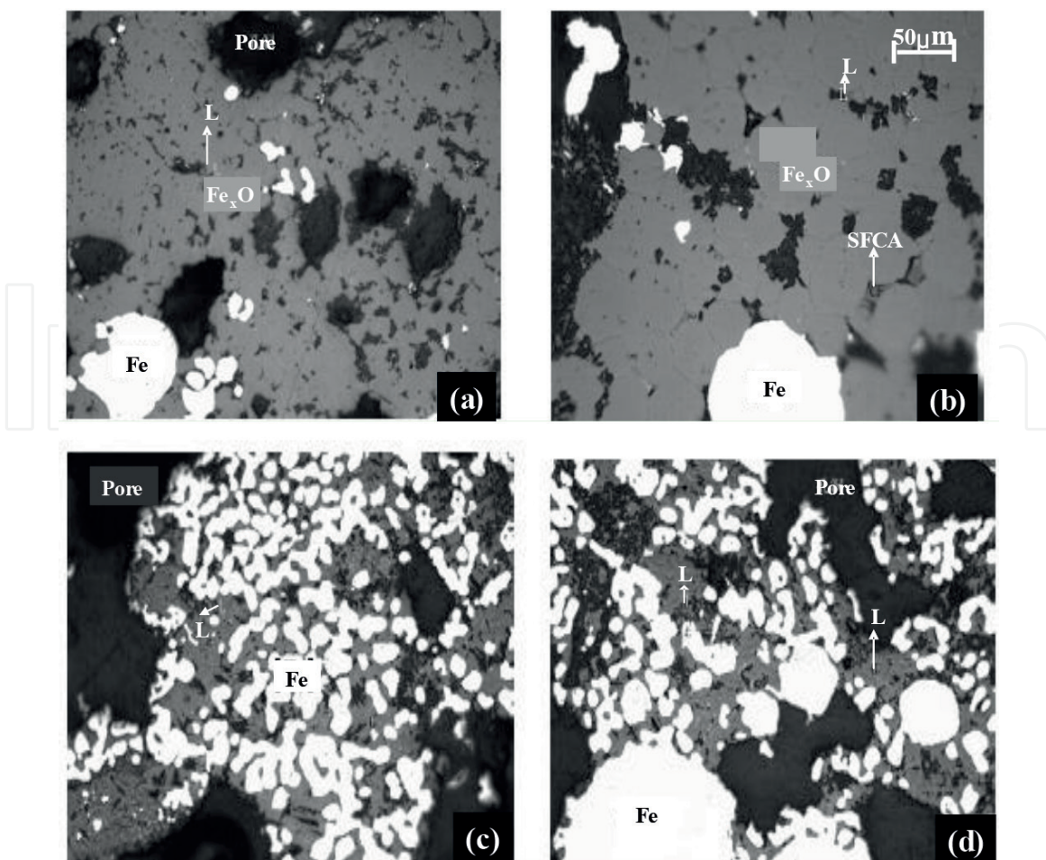
Figure 12. Optical reflecting microstructures of the reduced pellets, 200×: (a) and (b) interior and (c) and (d) exterior. L: silicate, SFCA: composite calcium ferrite, Fe: metallic iron, and \text{Fe}_x\text{O} : wustite.
