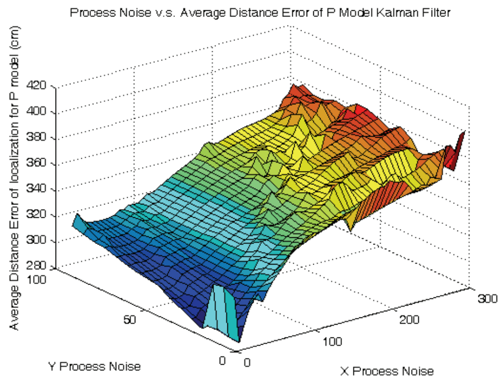
Fig. 12. Process noise versus localization error for P model using a maximum error threshold of 10,000 cm
