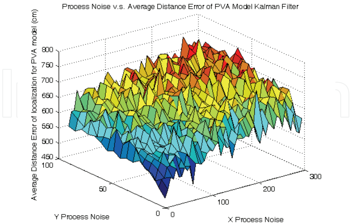
Fig. 14. Process noise versus localization error for PVA model using a maximum error threshold of 10,000 cm
