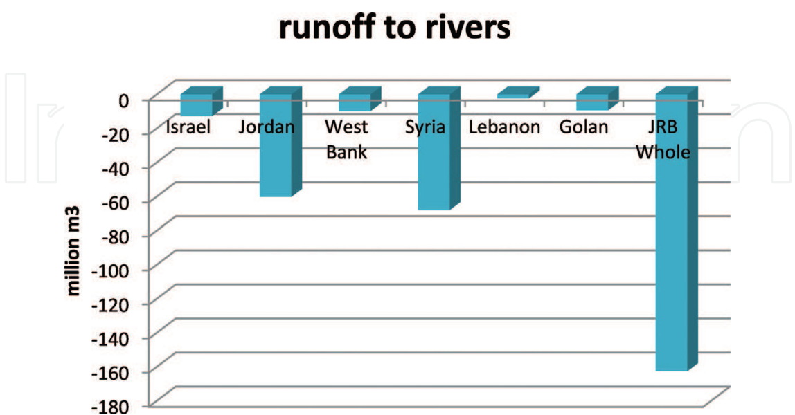
Figure 6. Impact of climate change on run-off.
