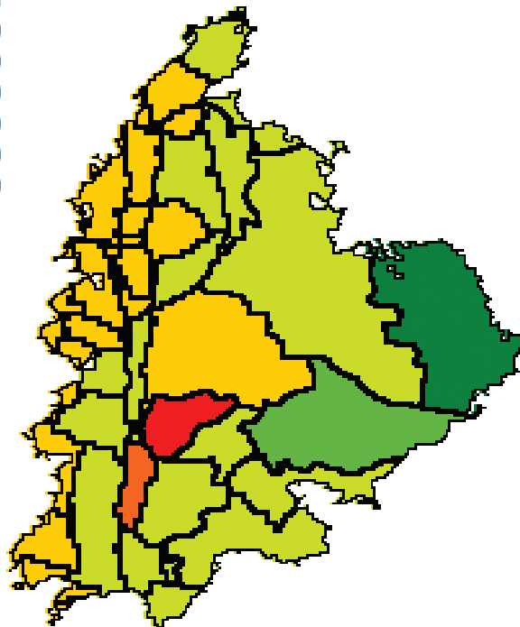
Figure 4. Rainfall in 2050: Predicted change relative to present conditions.
