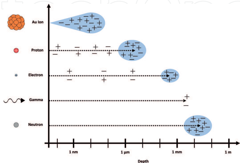
Figure 1. Illustration of the relative average interaction length scales for various types of radiation at an energy of 1 MeV incident on gold. Dotted lines indicate the mean free path of the incident particles. Positive and negative signs indicate ionization events, while blue highlighted areas denote displacement damage cascades.
