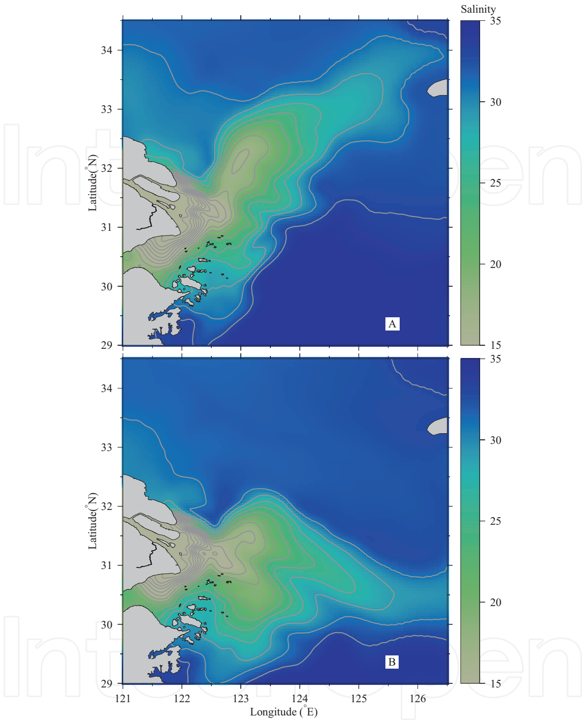
Figure 9. Tidally averaged surface salinity during spring tide under (A) southeasterly wind (i.e., Exp5) and (B) southwesterly wind (i.e., Exp6).
