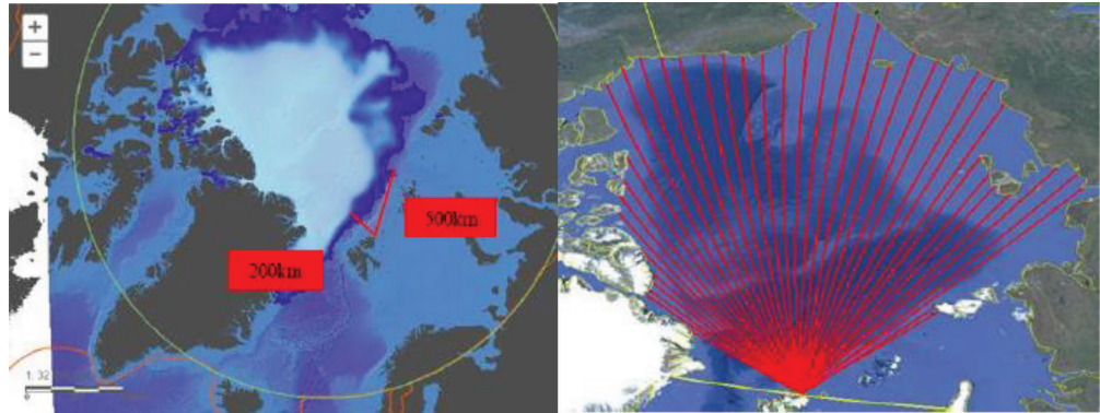
Figure 3. Present maximum and minimum available fetch lengths north of Svalbard during early autumn periods (left). Future fetch lengths available in a free ice Arctic Ocean, between 320 and 55° in steps of 2.5°.
