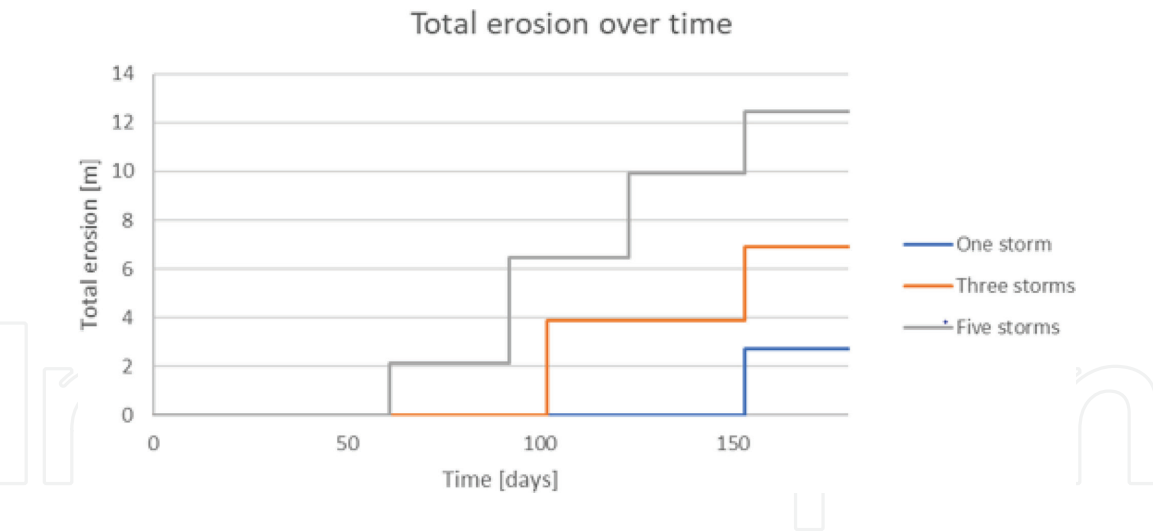
Figure 4. The effect of number of storms on the total erosion as a function of time [10].
