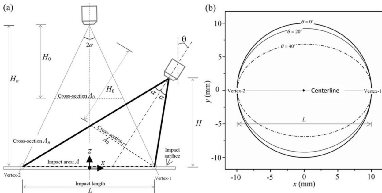
Figure 3. (a) The 2D geometry is on the central plane (z-x plane) of the cone perpendicular to the impacted surface (x-y plane). The positioning of the nozzle is determined by inclination angle \theta and spray height H . H_n is the required spray height by normal impact to cover a given impact length L . (b) Impact area with constant impact length L formed by the spray inclined at different angles \theta [21].
