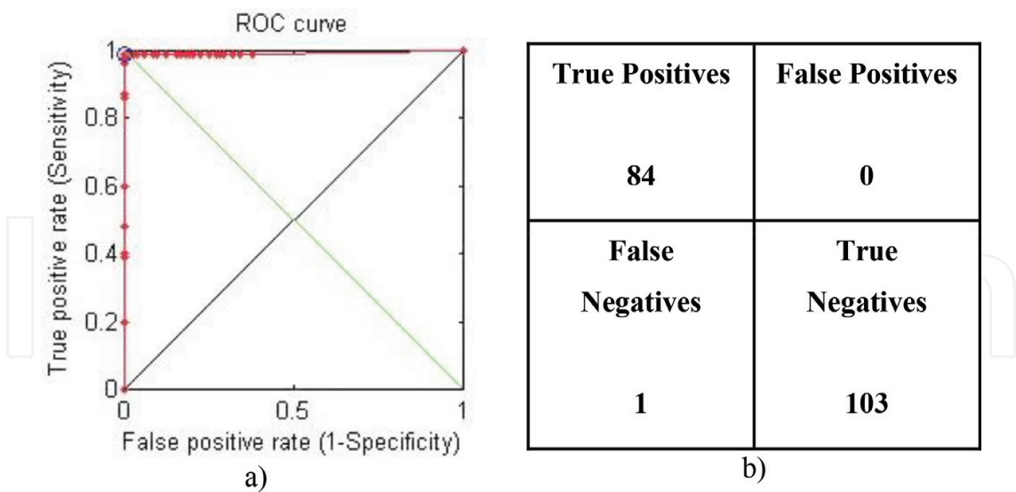
Figure 9. (a) ROC curve of the overall fuzzy system evaluation and (b) confusion matrix for 188 data evaluated.
