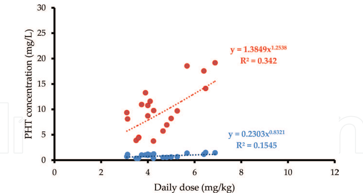
Figure 4. Relationship between the normalized dose of PHT and plasma concentration (in red) and salivary concentration (in blue) for Comitoína®.
