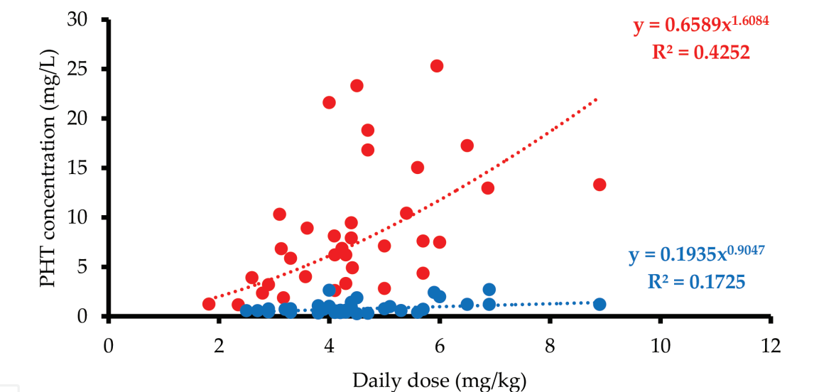
Figure 5. Relationship between the normalized dose of PHT and plasma concentration (in red) and salivary concentration (in blue) for Antepil®.
