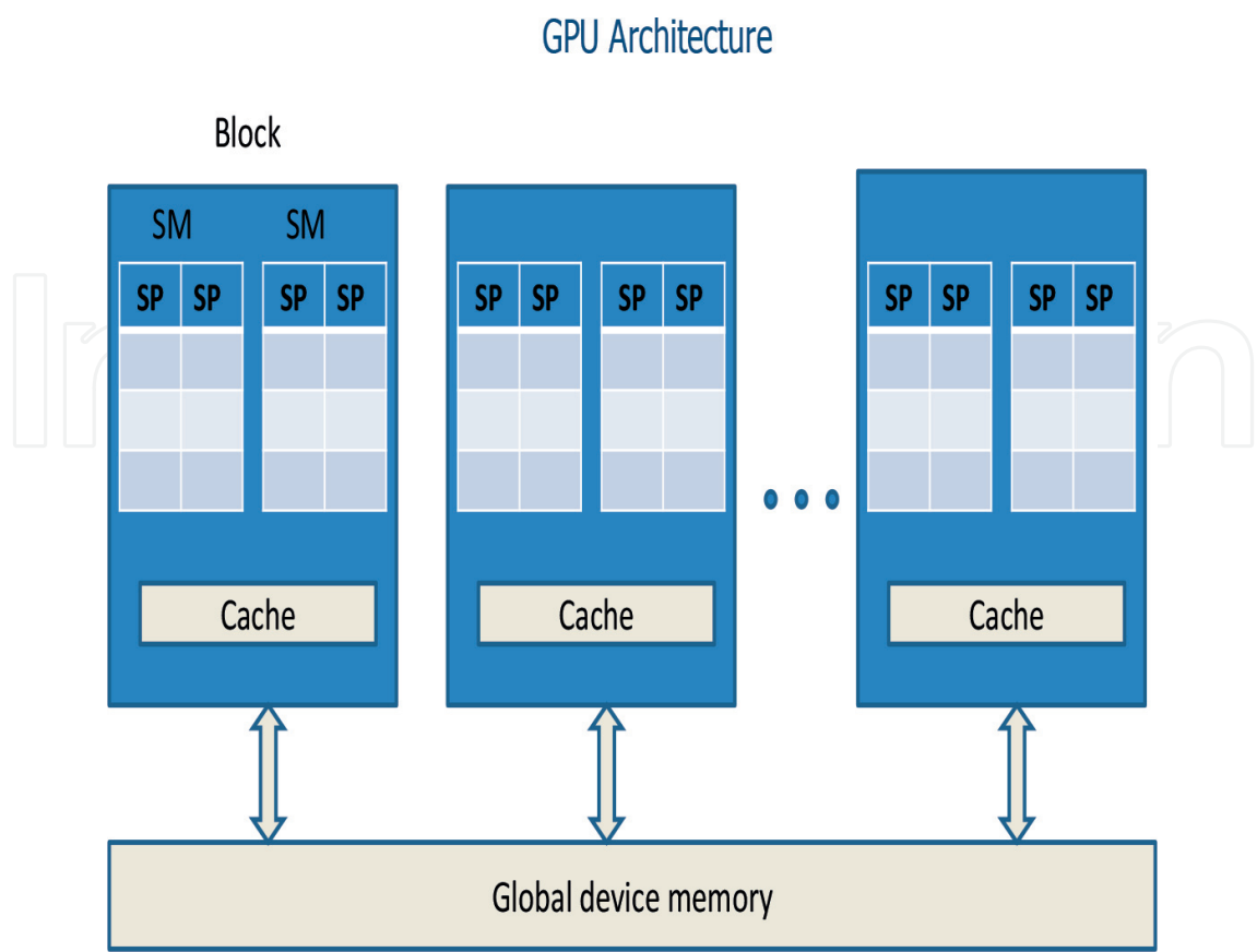
Figure 8. Architecture of a CUDA-capable GPU.
