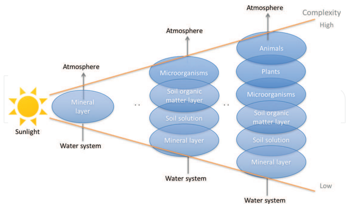
Figure 1. Axial hierarchy of emergence and evolution of land ecosystems.
