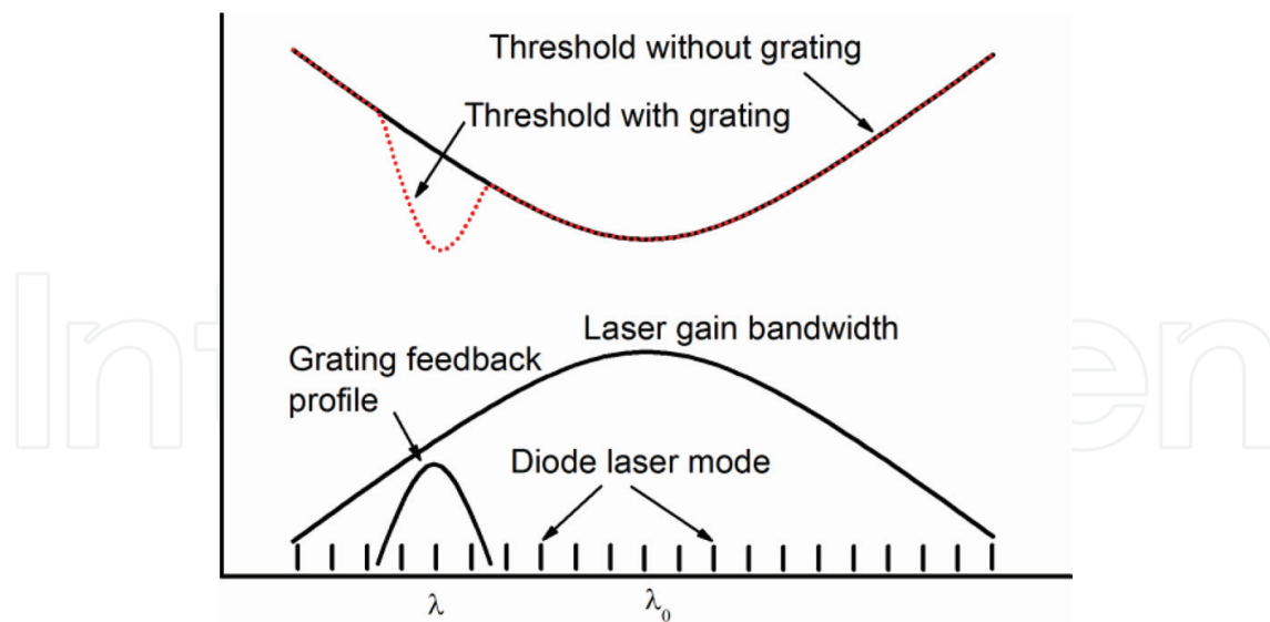
Figure 9. Schematic diagram of the gain and threshold with and without grating feedback. The grating feedback profile is also shown.
