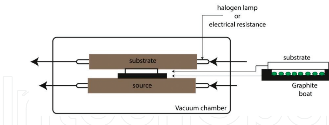
Figure 3. A simple CSVT system. This system generates a temperature gradient between the substrate and source where the temperature of the source is higher. For this temperature difference, the material is deposited on the substrate; the variable is substrate and source temperature.
