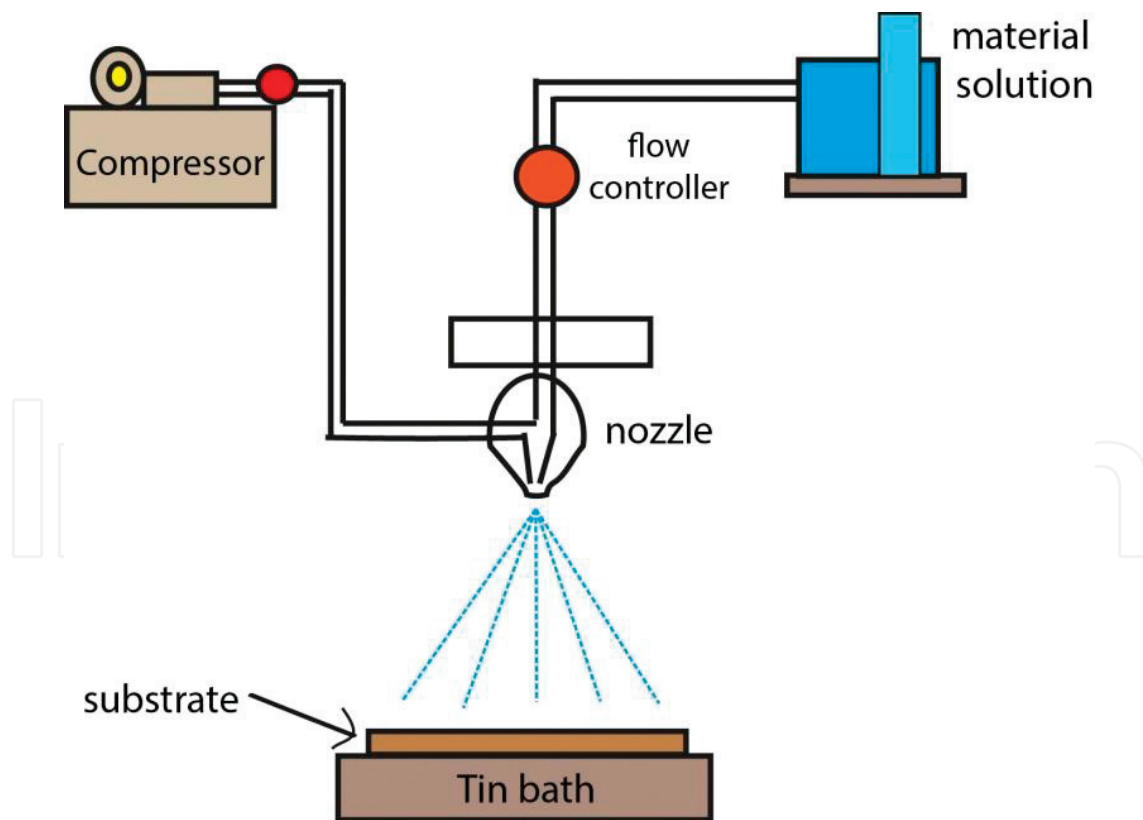
Figure 6. Spray pyrolysis system. The solution moves through the tubes to meet the air in the nozzle to produce the spray, which arrives on the substrate that is heated to deposit the material. The variables are concentration solution, pressure, and the substrate temperature.
